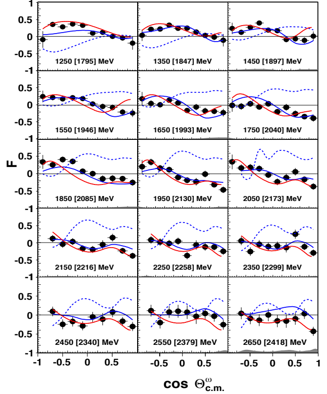
FIG. 2. First-time measurement of the beam-target asymmetry F in \vec{\gamma}p \rightarrow p\omega . Shown are distributions in 100-MeV-wide incident-photon energy bins (labeled as E_\gamma [W]) as a function of \cos \Theta_{\text{c.m.}}^\omega in the center-of-mass frame. Each data point has been assigned its statistical uncertainty, whereas the gray band at the bottom of each panel represents the absolute systematic uncertainties due to the background subtraction. The blue and red solid curves show the BnGa PWA solution and fits by Wei et al. [23], respectively. The blue dashed curve denotes an earlier BnGa solution [26].
