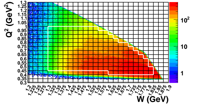
FIG. 13. (colors online) Q^2 versus W distribution populated with selected double-pion events. The cross section was calculated in 2D cells within the white boundaries.
