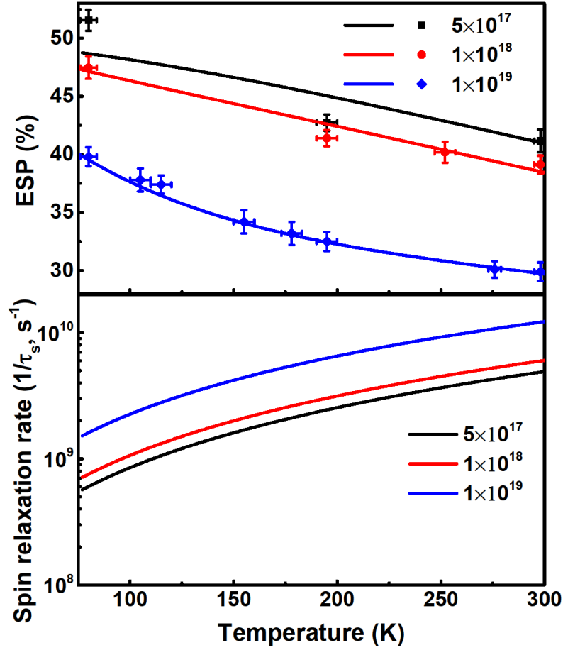
Figure 5: (top) Maximum ESP versus sample temperature and dopant density (the wavelength of illumination was allowed to vary to provide peak polarization). Dots are experimental data and lines represent fits based on calculations using Equations 2, 3, and 4. Vertical error bars are statistical. Horizontal error bars are attributed to uncertainty in sample temperature. (bottom) Calculated values of spin relaxation rate versus sample temperature and dopant density.
