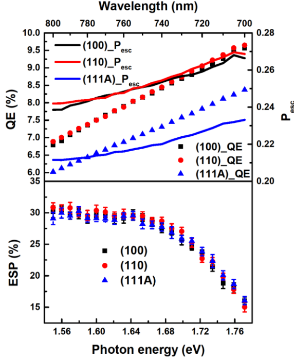
Figure 7: QE, Escape Probability and ESP of bulk GaAs with three different cleave planes, Zn dopant concentration of 1 \times 10^{19} \text{ cm}^{-3} measured at room temperature. Error bars are statistical. The plots of escape probability P_{\text{esc}} are based on measured values of QE, and inferred values of reflectivity, absorption coefficient, and electron diffusion length as described in Section II.
