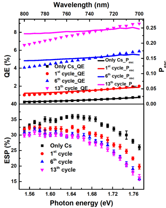
Figure 6. QE, Escape Probability and ESP for bulk GaAs (110 cleave plane) with dopant concentration of 1 \times 10^{19} \text{ cm}^{-3} as a function of surface activation layer. Cycle number refers to the number of applications of Cs and F. Error bars are statistical. The plots of escape probability P_{esc} are based on measured values of QE, and inferred values of reflectivity, absorption coefficient, and electron diffusion length as described in Section II.
