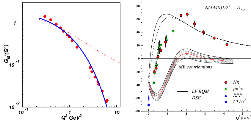
Fig. 4 (Color Online) Insight into the resonance structure and strong QCD dynamics from the experimental results on the magnetic p \rightarrow \Delta(1232)3/2^+ transition form factor (left) [16] and the A_{1/2} electrocoupling of the N(1440)1/2^+ resonance (right) [16,32,33]. The red dashed and blue solid curves in the left panel correspond to the computation of the magnetic p \rightarrow \Delta(1232)3/2^+ transition form factor starting from the QCD-Lagrangian within DSE by employing a simplified contact qq -interaction (frozen quark mass) and a realistic qq -interaction (running quark mass), respectively [18]. In the right panel the DSE computation of the A_{1/2} electrocoupling of the N(1440)1/2^+ resonance with a realistic qq -interaction and the same running quark mass as employed in the successful evaluations of nucleon elastic and magnetic p \rightarrow \Delta(1232)3/2^+ form factors is shown by the dashed line [19]. The result from a novel light front quark model [7,8], which incorporates a momentum dependent dressed quark mass, is shown by the solid line. The shadowed area represents the meson-baryon cloud contribution inferred from the experimental results on the A_{1/2} electrocoupling of the N(1440)1/2^+ resonance and the DSE evaluation [19] of the quark core contribution.
