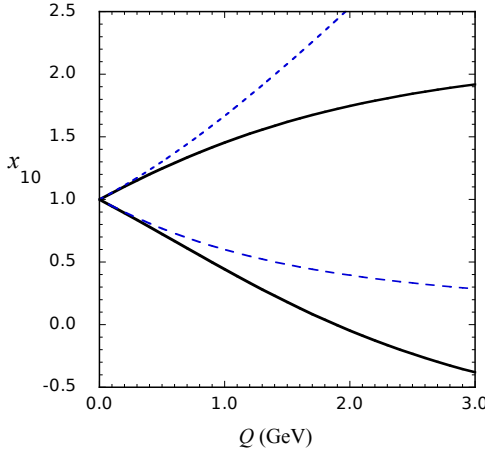
FIG. 15. Plot of the maximum and minimum of x_{10} as a function of Q . The black solid lines show the maximum and minimum, including boost effects, as obtained from Eq. (A31); the blue dashed lines are the maximum and minimum without boost effects as obtained from Eq. (3.4).
