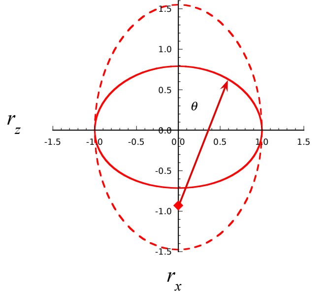
FIG. 24. Locus of the points \{r_z^b, r_\perp^b\} of Eq. (A28) (the solid line ellipse) compared to \{r_z, r_\perp\} of Eq. (A17) (the dashed-line ellipse, identical to the one shown in Fig. 23) as a function of \theta . The diamond reference point near r_z \sim -1 is the point from which the magnitude of the transformed momentum is measured. I choose Q = 2 GeV and k = 400 MeV for this example.
