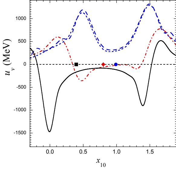
FIG. 16. The invariants u_v and w_v defined in Eq. (3.5) for the favored model WJC2, shown as a function of x_{10} for four fixed momenta: k = k(1) \simeq 0.527 MeV (blue long dashed lines), k = k(10) \simeq 84.0 MeV (blue short dashed lines), k = k(23) \simeq 450.3 MeV (red dot-dashed line), and k = k(32) \simeq 960.8 MeV, where k(n) is the n th gauss point in the mapped grid of 60 points. The values of x_{10} when particle 2 is on shell are shown for k(10) (solid blue circle), k(23) (solid red diamond), and k(32) (solid black square).
