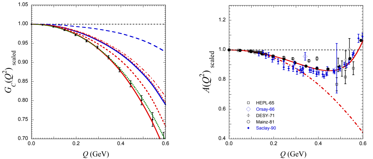
FIG. 20. Study of relativistic effects. The left panel is scaled by G_C^{\text{NR}} given in Eq. (4.1); the right panel is scaled by (G_C^{\text{NR}})^2 . In both panels the small black dots are the Sick GA (with error bars) and the thick solid red lines are the predictions for model 2D. The other curves are discussed in the text.
