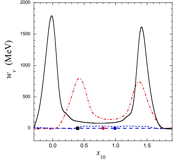
FIG. 16. The invariants u_v and w_v defined in Eq. (3.5) for the favored model WJC2, shown as a function of x_{10} for four fixed momenta: k = k(1) \simeq 0.527 MeV (blue long dashed lines), k = k(10) \simeq 84.0 MeV (blue short dashed lines), k = k(23) \simeq 450.3 MeV (red dot-dashed line), and k = k(32) \simeq 960.8 MeV, where k(n) is the n th gauss point in the mapped grid of 60 points. The values of x_{10} when particle 2 is on shell are shown for k(10) (solid blue circle), k(23) (solid red diamond), and k(32) (solid black square).
