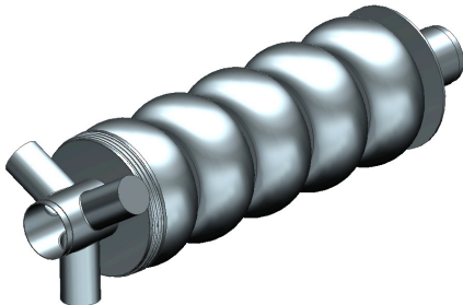
Fig. 6. Concept for ERL cooler cavity.
