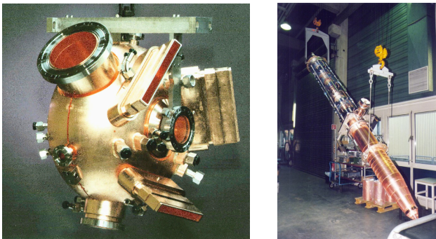
Figure 2. PEP-II RF cavity and 1.2 MW klystron.
