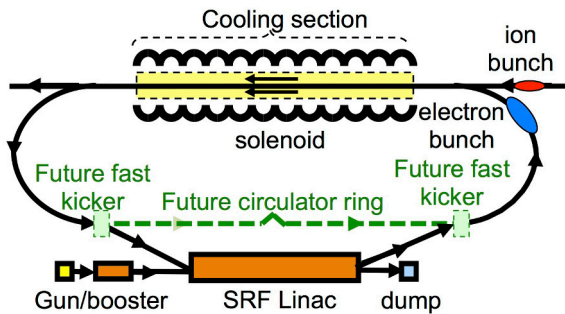
Fig. 5. schematic of bunched beam cooler with option for future recirculation.
