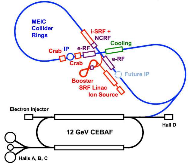
Figure 1. Schematic layout of figure-8 MEIC.
