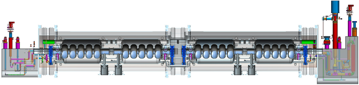
Figure 7: Concept for a versatile modular cryostat to house various MEIC SRF cavities (ERL concept shown).
