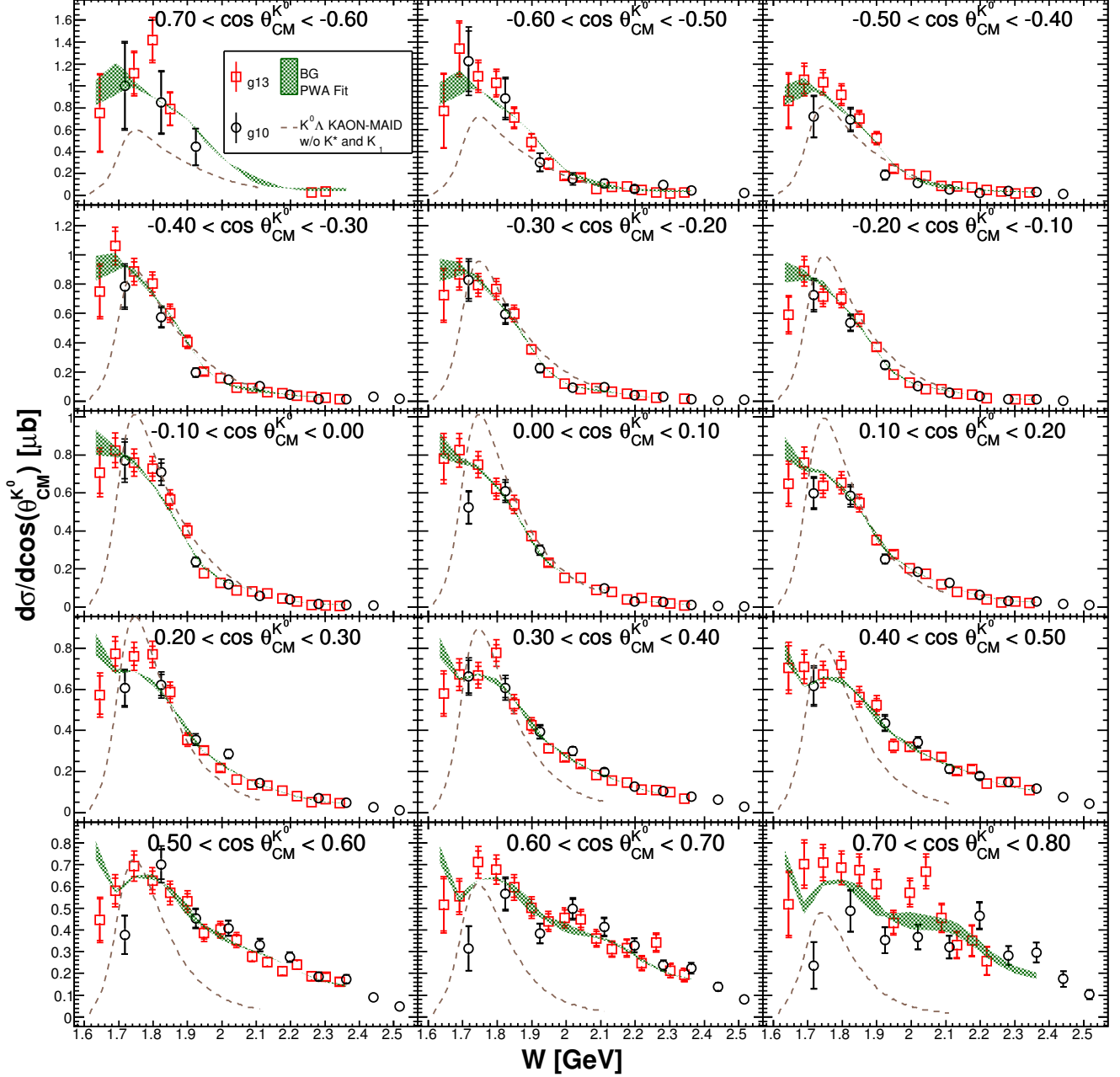
FIG. 12. The g10 (circles) and g13 (squares) differential cross sections as a function of W (GeV) for each \cos \theta_{c.m.}^{K^0} . The KAON-MAID model (dashed line) is shown, assuming no contributions from the K^*(892) and K_1(1270) , along with the differences between the two Bonn-Gatchina K^0\Lambda fits (shaded curve). The inner error bars represent the statistical uncertainty. The outer error bars are the statistical and systematic uncertainties added in quadrature.
