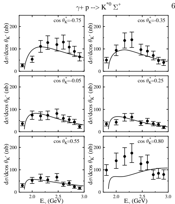
FIG. 5: Cross sections for the reaction \gamma p \rightarrow K^{*0}\Sigma^+ as a function of energy for the angular bins shown. The curves are from the same model as in the previous figure. Error bars include systematic uncertainties.
