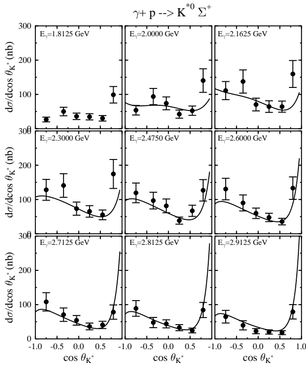
FIG. 4: Cross sections for the reaction \gamma p \rightarrow K^{*0}\Sigma^+ as a function of angle for the energy bins shown. The curves are from the model of Zhao [4] using vector and tensor couplings adjusted to give the best fit to the data. Error bars include systematic uncertainties.
