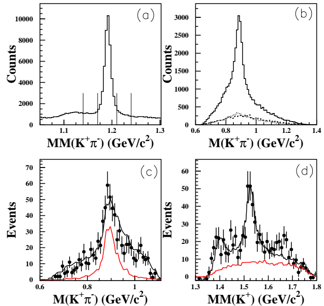
FIG. 2: (a) Missing mass for the \gamma p \rightarrow K^+\pi^- X reaction summed over all angles and photon energies. (b) Invariant mass of the K^+\pi^- system, with the same event selection, for events in the \Sigma^+ peak (solid) and the sideband regions (dashed and dotted) shown in (a). (c) M(K^+\pi^-) for E_\gamma = 2.24\text{-}2.36 GeV and -0.2 < \cos\theta_{K^*} < 0.1 showing the full fit (black) and the K^{*0} peak component (red). (d) MM(K^+) showing the \Lambda(1520) and other hyperon peaks (see Fig. 1, right) along with the curves as in (c).
