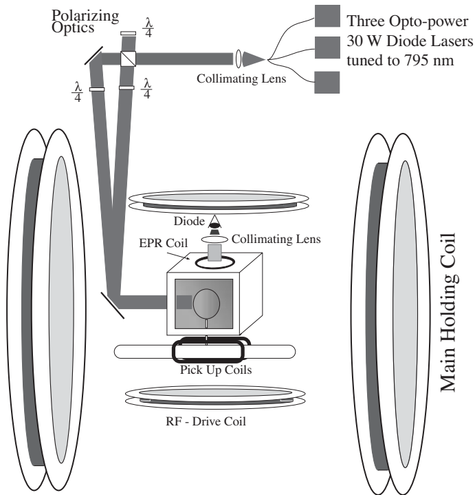
Fig. 21. Schematic lay-out of the spin-exchange polarized ^3\text{He} target. For clarity, only one set of Helmholtz coils is shown.
