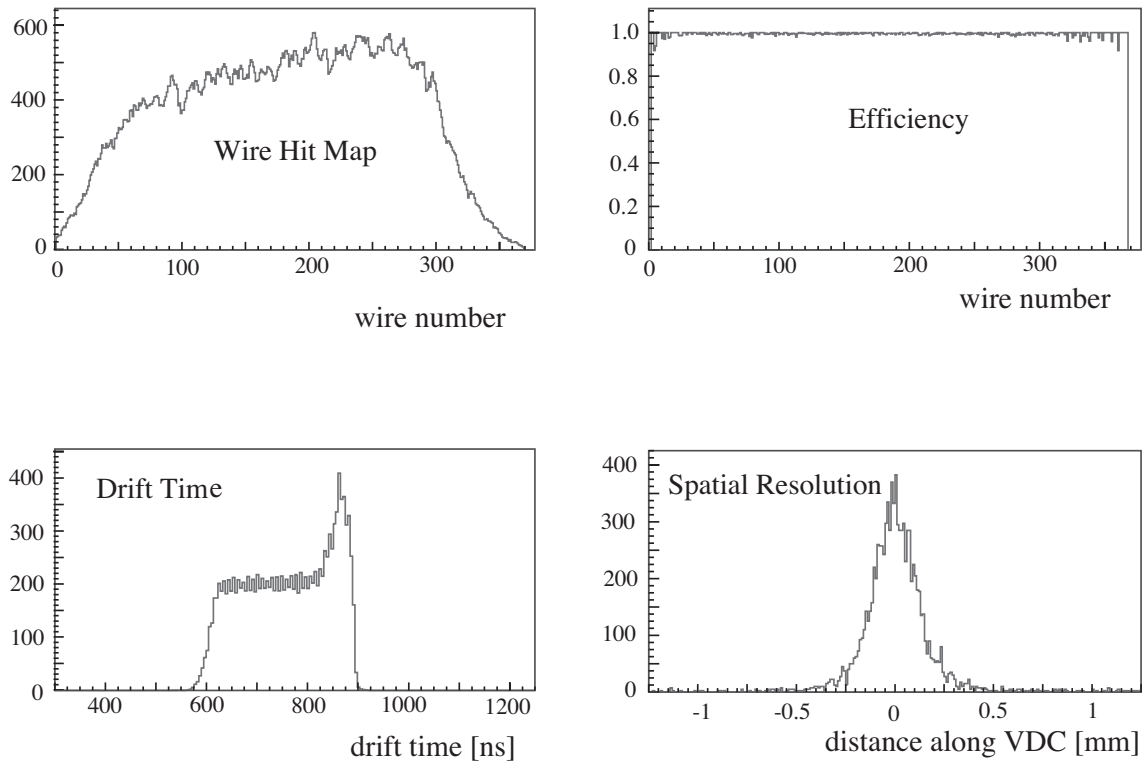
Fig. 8. Typical on-line results of the analysis of one VDC to monitor its performance: top left, response as a function of the wire number; top right, wire efficiency as a function of the wire number; bottom left, drift-time spectrum (short drift times occur at large TDC values); bottom right, spatial resolution for events with hits in six adjacent wires.
