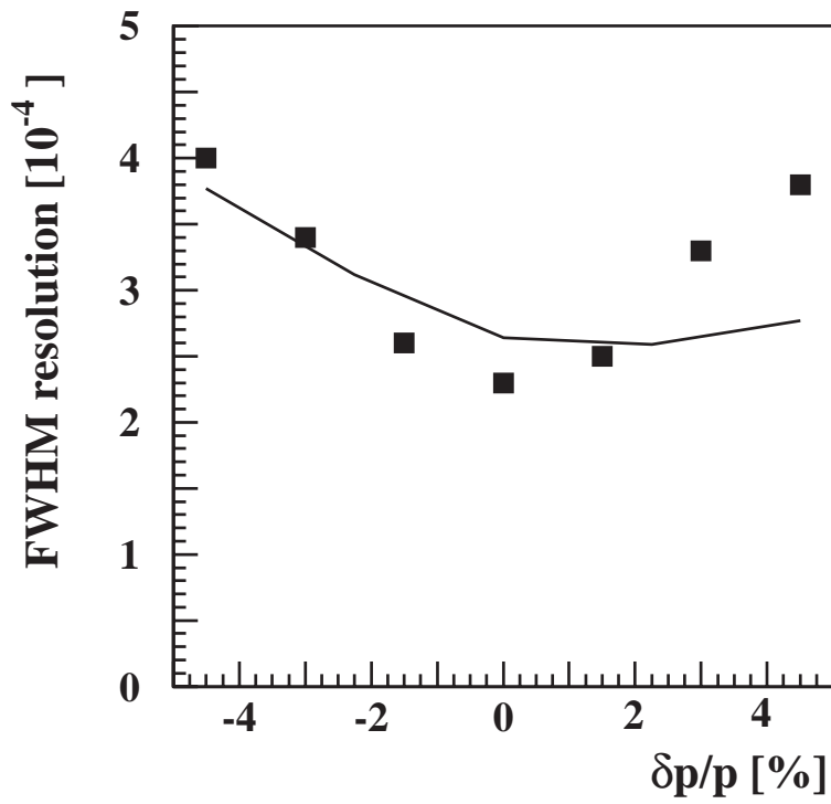
Fig. 29. The FWHM momentum resolution \delta p/p measured in the reaction ^{12}\text{C}(e, e') as a function of the momentum of the scattered electron. The curve represents the result of a simulation, taking into account the optical properties of the HRS device and multiple scattering effects.
