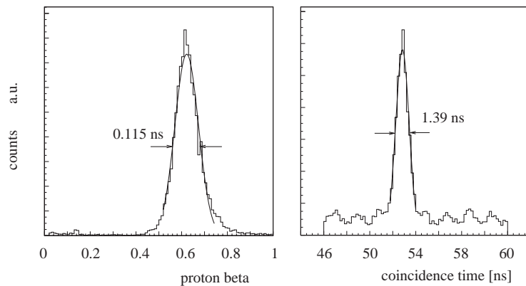
Fig. 9. Velocity distribution (left) in units of \beta = v/c for protons and the coincidence time spectrum (right) between the two HRS, as measured with the two scintillator planes. The small peaks in the right figure show the time structure of the primary electron beam.
