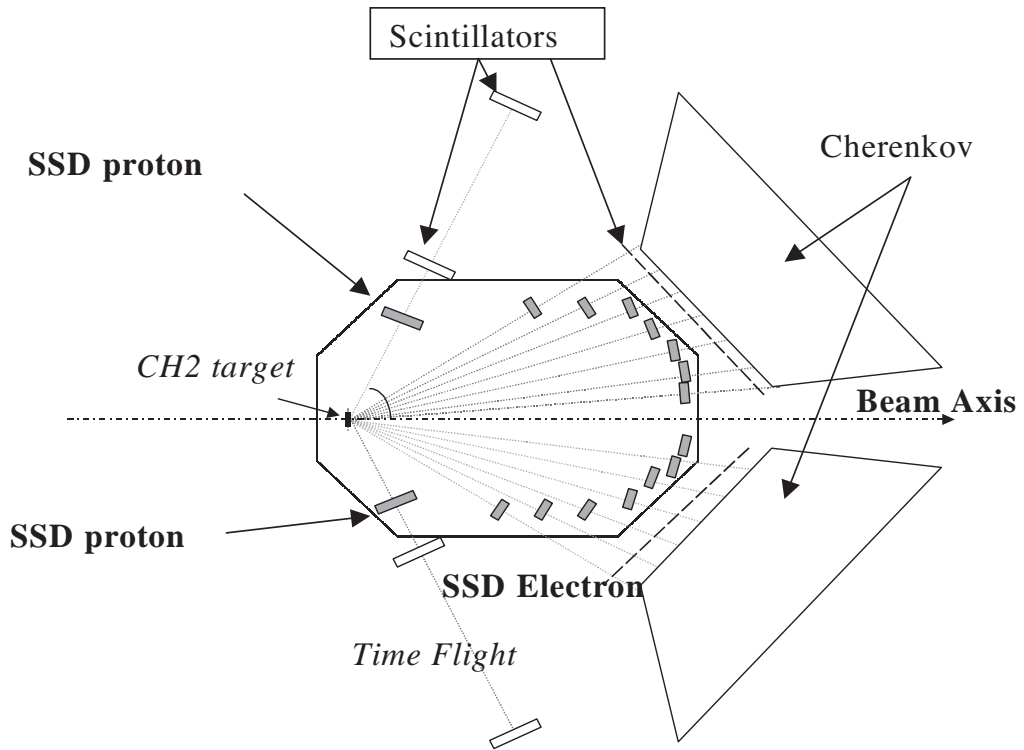
Fig. 17. Schematic lay-out of the eP energy measurement system, showing the arrangement of its components, the polyethylene (CH2) target, the Cherenkov detectors, the silicon-strip detectors (SSD) for protons and electrons and the scintillator detectors, used for time-of-flight measurements.
