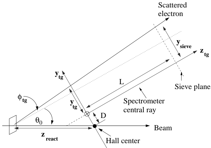
Fig. 27. Coordinates for electrons scattering from a thin foil target. \mathbf{L} is the distance from Hall center to the sieve plane, while \mathbf{D} is the horizontal displacement of the spectrometer axis from its ideal position. The spectrometer central angle is denoted by \theta_0 . Note that x_{tg} and x_{sieve} are vertically down (into the page)
