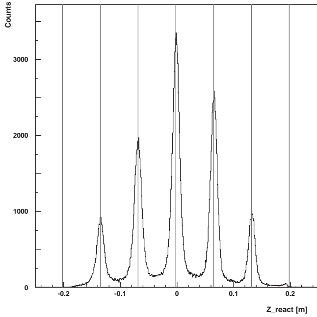
Fig. 26. Reconstructed position along the beam line ( z_{react} ) for 860 MeV electrons scattered from a set of ^{12}\text{C} foil targets. The lines indicate the expected positions of the foils. The spectrometer was set at 16^\circ to the beam. The z_{react} resolution for the central foil is 1.5 cm (FWHM). Note that this corresponds to about 4 mm (FWHM) resolution in the y_{tg} direction.
