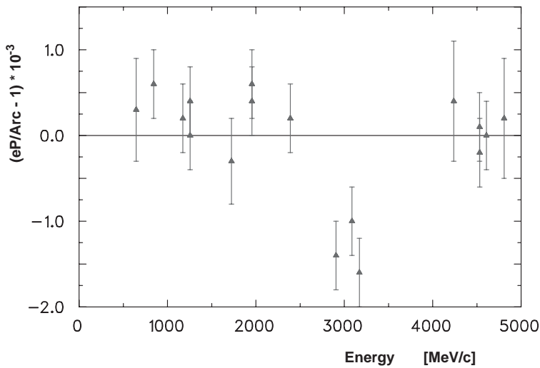
Fig. 18. A comparison of energy measurements with the Arc and the eP system as a function of the electron beam energy.
