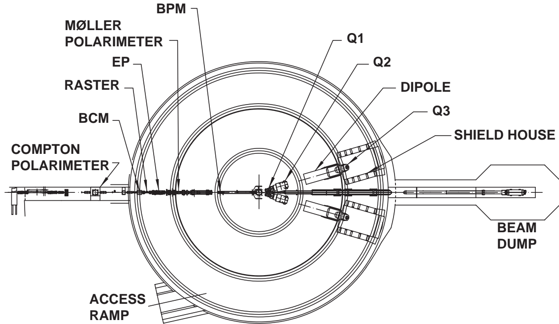
Fig. 16. Schematic lay-out of Hall A, indicating the location of the Compton and the Møller polarimeters, the raster, the EP energy measurement system, the beam current monitors (BCM) and the beam position monitors (BPM) upstream of the target. Also indicated are the locations of the components of one of the high-resolution spectrometers (Q1, Q2, dipole, Q3 and shield house) and of the beam dump and the truck access ramp.
