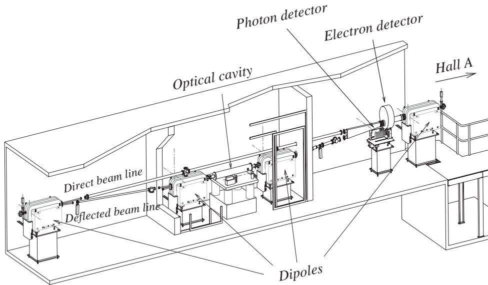
Fig. 20. Schematic lay-out of the Compton polarimeter, showing the four dipoles of the chicane, the optical cavity and the photon and electron detector.
