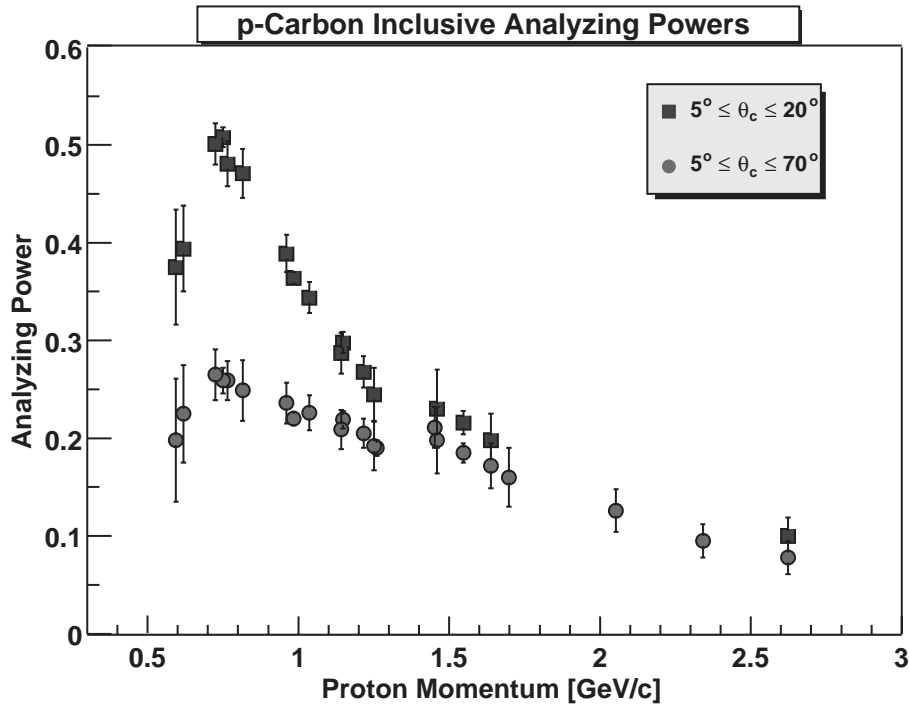
Fig. 15. The average analyzing powers of the carbon analyzer as a function of proton momentum. Solid squares are averages over scattering angles from 5^\circ to 20^\circ and the solid circles for those from 5^\circ to 70^\circ .
