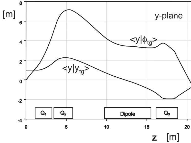
Fig. 4. First-order trajectories in a High Resolution Spectrometer. The top (bottom) graph shows the evolution of the first-order matrix elements in the horizontal (vertical) plane, as a function of the trajectory length. The location of the four magnetic elements is also indicated.
