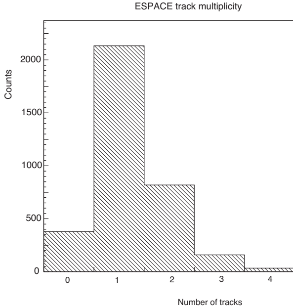
Fig. 24. Typical VDC track multiplicity determined by ESPACE in a high-rate environment (200 kHz of electron singles triggers).
