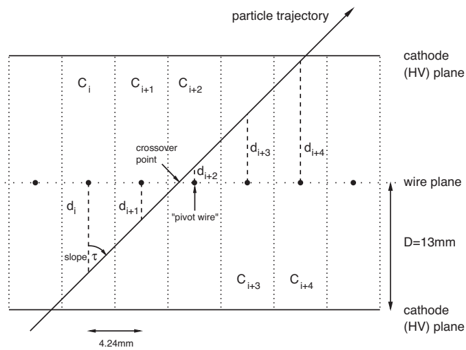
Fig. 23. A typical cluster of hits in a VDC plane. C_i denotes the i -th wire cell, and d_i represents the perpendicular (effective) drift distance within that cell. The i -th cell is defined as the region within which ions drift to the i -th wire. By symmetry, the cell boundaries lie halfway between wires. The wire spacing is 4.24 mm. The separation between cathode high-voltage and wire planes is approximately 13 mm. The HV planes are held at a potential of approximately -4 kV, while the wires are effectively grounded.
