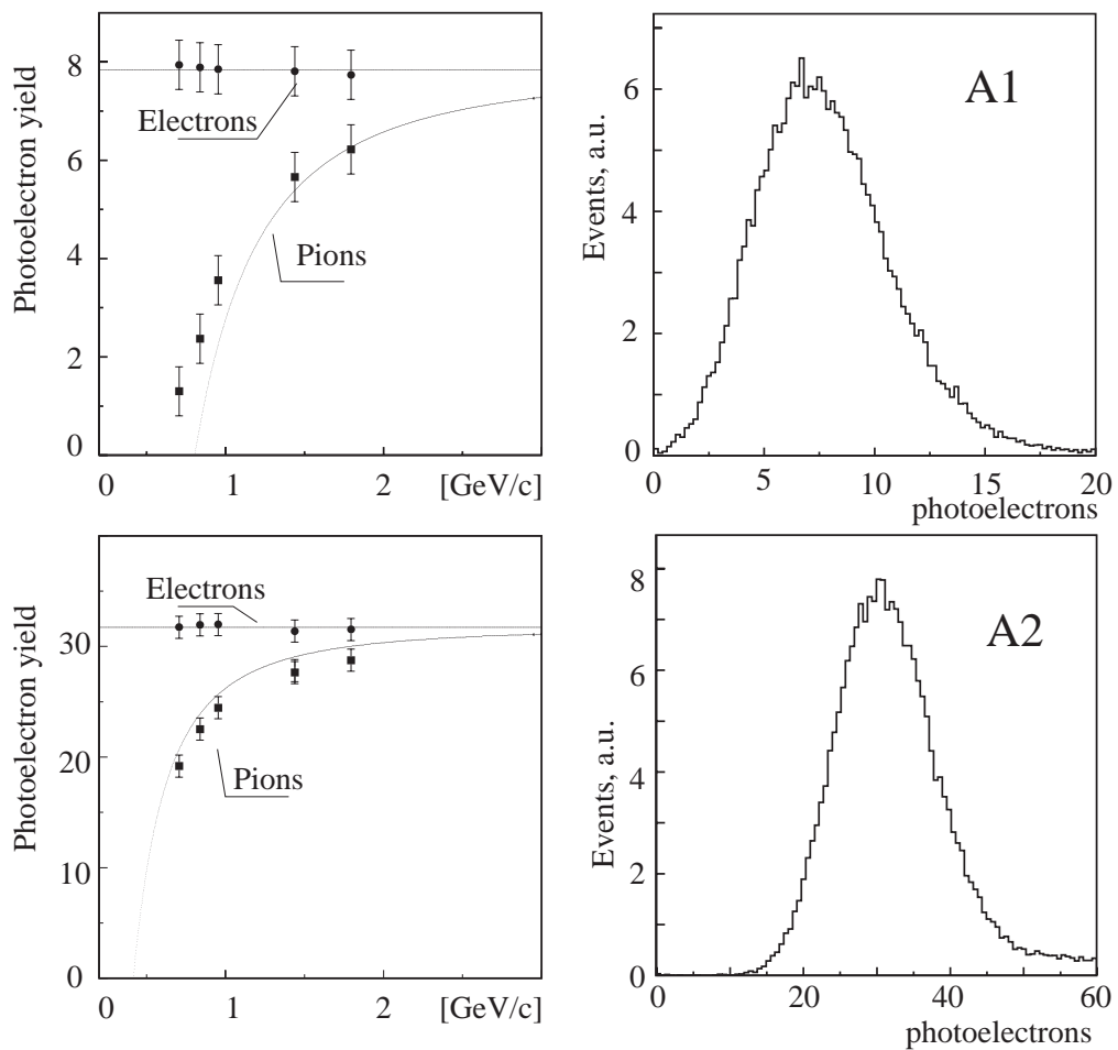
Fig. 12. The photo-electron yield vs particle momenta for A1 and A2 detectors (left) and examples of spectra for 2 GeV electrons (right). The curves indicate the expected photoelectron yield for the different particles as a function of momentum.
