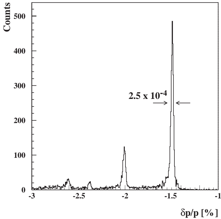
Fig. 28. The momentum of the scattered electron in the ^{12}\text{C}(e, e') reaction, indicating a FWHM of 2.5 \cdot 10^{-4} at \delta p/p = -1.5\% . The beam energy was 845 MeV, the scattering angle 16^\circ . The observed momentum resolution is consistent with the design value of 1 \times 10^{-4} when multiple scattering from the windows of the scattering chamber and of the HRS entrance are taken into account.
