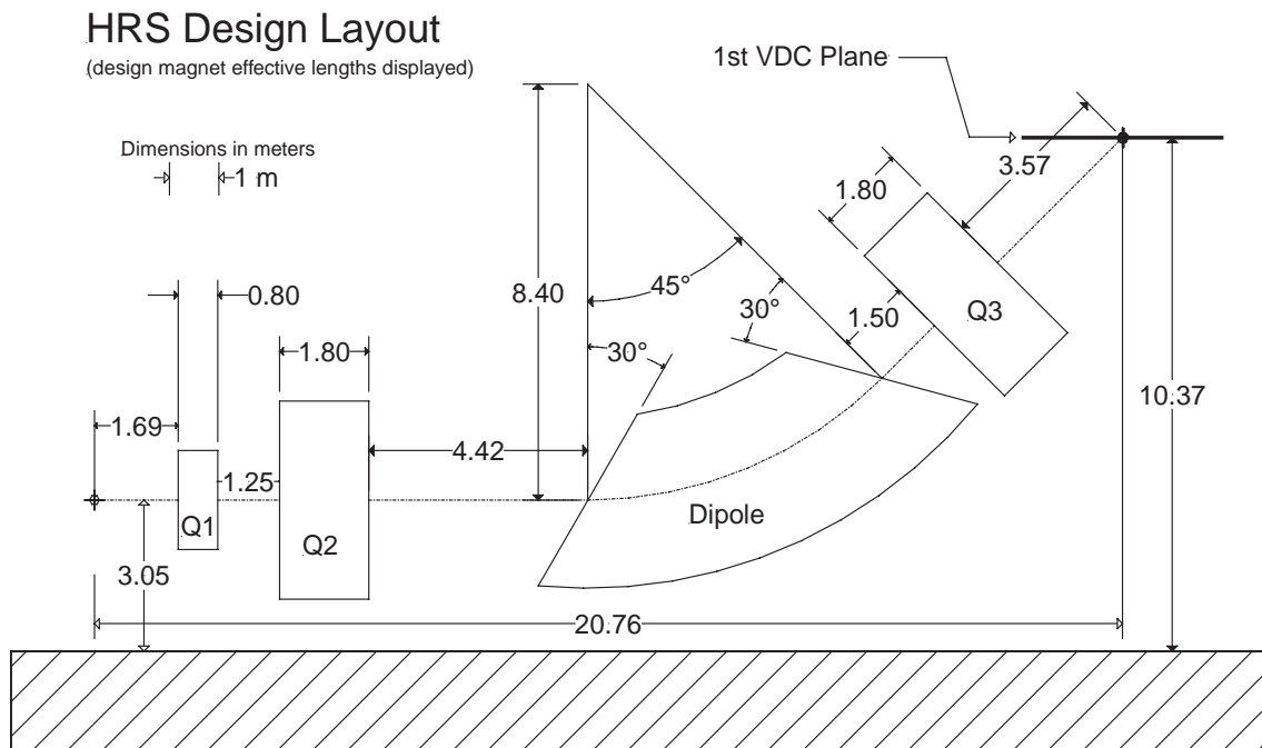
Fig. 3. Schematic lay-out of a HRS device, showing the geometrical configuration of the three quadrupole and the dipole magnets. Also shown is the location of the first VDC tracking detector.
