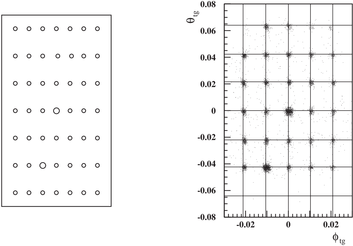
Fig. 5. Geometric (left) and reconstructed (right) configurations of the sieve slit. The large holes, which allow for an unambiguous identification of the orientation of the image at the focal plane, can be clearly identified in the right figure.
