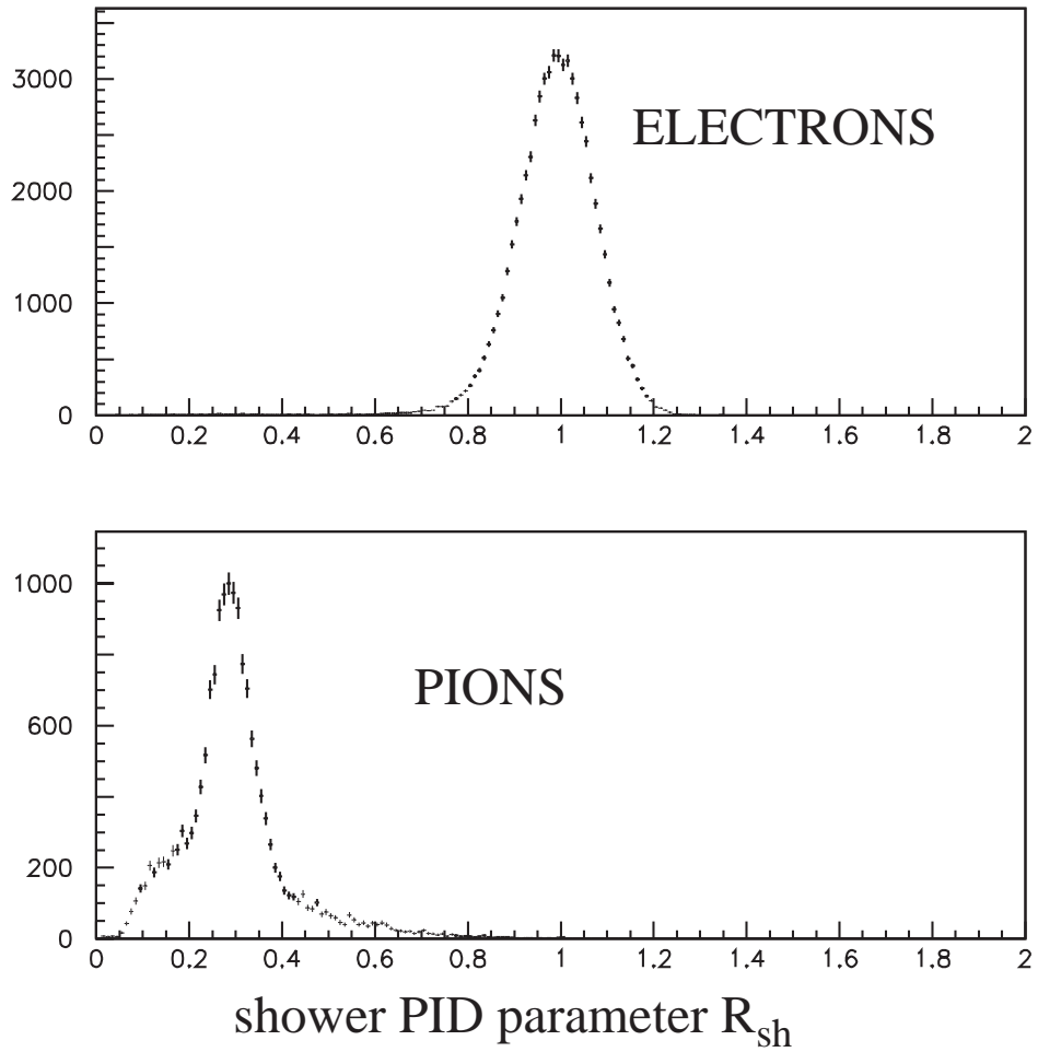
Fig. 11. The response function (defined in the text) of the HRS-R shower detector for pions and electrons at a momentum of 1.6 GeV/c.
