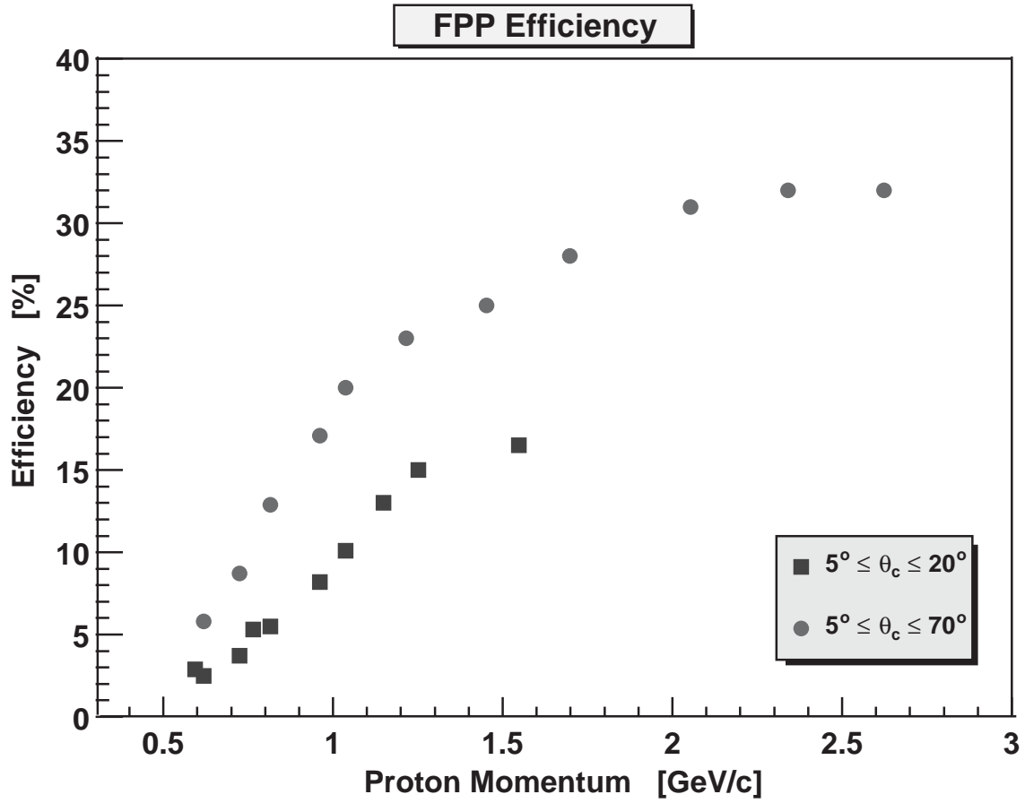
Fig. 13. The scattering efficiency of the FPP as a function of proton momentum for scattering angles from from 5^\circ to 20^\circ (solid squares) and for 5^\circ to 70^\circ (solid circles). The thickness of the analyzer was varied with momentum as described in the text.
