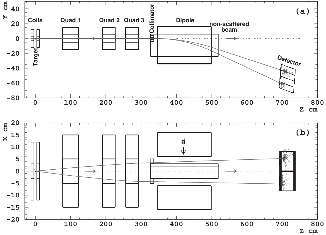
Fig. 19. Layout of the Møller polarimeter, (a) presents a side view while (b) presents a top view. The trajectories displayed belong to a simulated event of Møller scattering at \theta_{CM} = 80^\circ and \phi_{CM} = 0^\circ , at a beam energy of 4 GeV.
