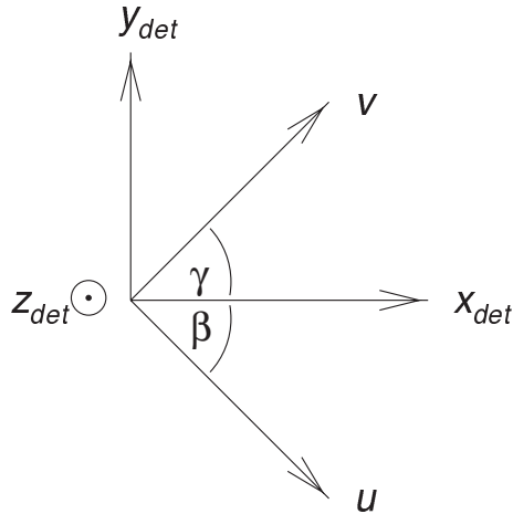
Fig. 25. Top view of the wire plane and VDC detector coordinate systems. The u and v axes are perpendicular to the wires of the U and V planes, respectively, and point in the direction of increasing wire numbers. The x -axis lies in the horizontal plane and points along the spectrometer dispersive direction (the long side of the VDC frame) such that x_{det} increases as momentum increases. z_{det} points vertically up, and y_{det} is oriented along the non-dispersive direction to form a right-handed coordinate system. The u and v -axes form angles \beta and \gamma with respect to the VDC x -axis. For the Hall A VDCs, \gamma = 45^\circ and \beta = -45^\circ .
