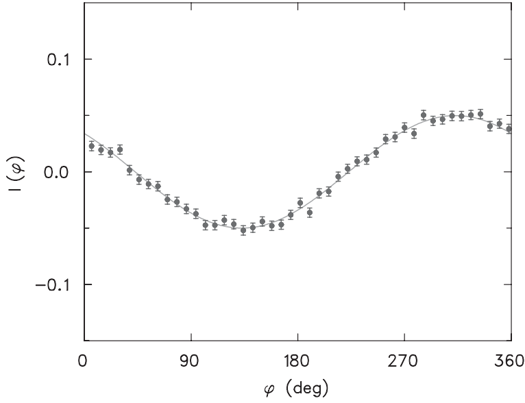
Fig. 14. The azimuthal distribution of protons scattered in the FPP in ep elastic scattering with 4.6 GeV incident electron energy and Q^2 = 3.5 \text{ (GeV/c)}^2 .
