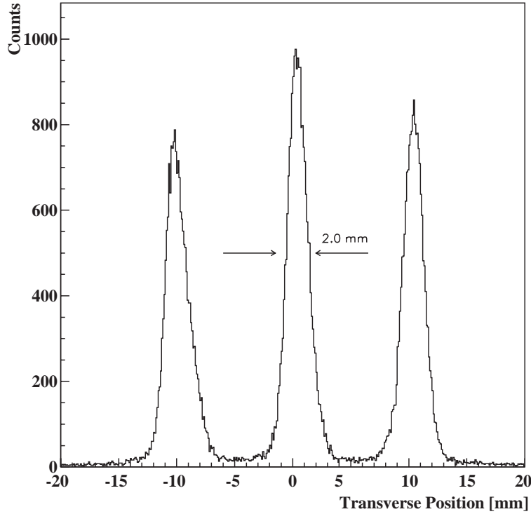
Fig. 22. The position of the three waterfall foils, reconstructed from the focal plane detector information.
