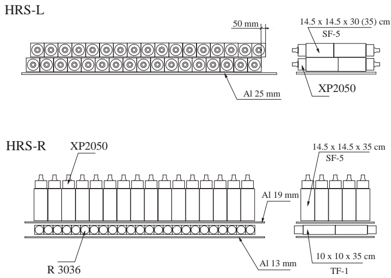
Fig. 10. Schematic lay-out of part of the shower detectors in HRS-L (top) and HRS-R (bottom). Particles enter from the bottom of the figure.
