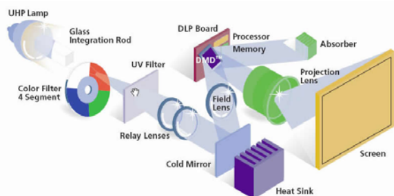
Figure 5: DLP™ display projection engine.
