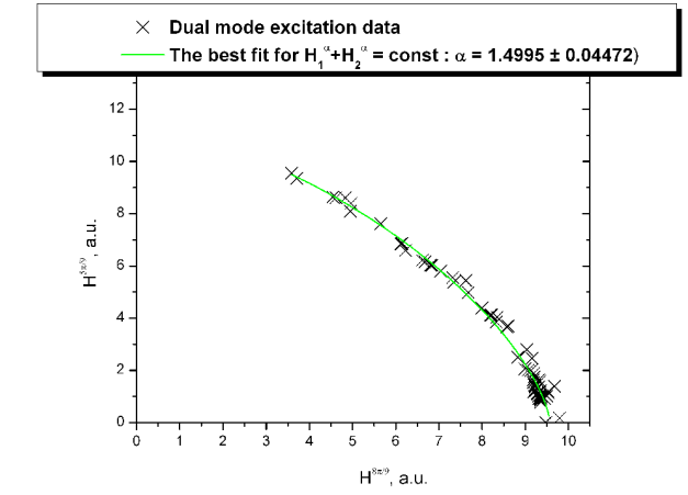
Figure 4: 8\pi/9 and 5\pi/9 dual mode excitation result. It was not possible to investigate the whole parameter space, because 5\pi/9 mode was limited by a defect other than the one limiting 8\pi/9 at 40.5 \text{ MV/m} . Black dots are measurement data. The green line is the best fit. The best fit exponent is 1.50 \pm 0.04 .
