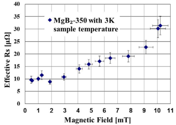
Figure 5: Effective surface resistance of MgB 2 -350 versus magnetic field at 3 K.
