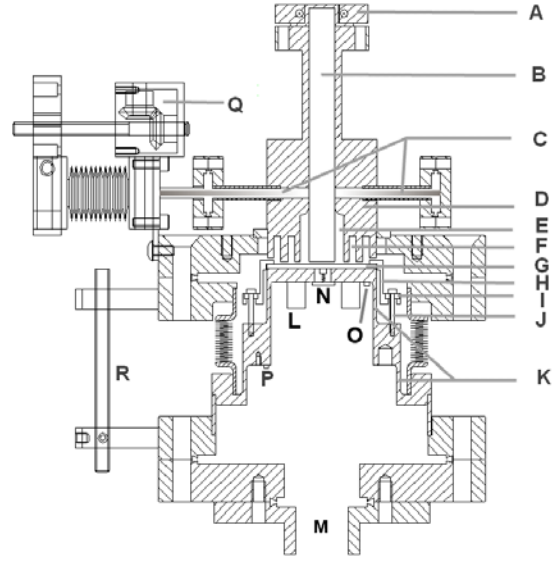
Figure 1: SIC system cross-section. A. Cap for sapphire rod, B. Sapphire rod, C. RF coupler, D. Nb cavity body, E. TE 011 cavity, F. Double choke joints, G. Sample on top of copper sample holder, H. Stainless steel sample clamp, I. G-10 washer, J. Aluminium bolt, K. Upper and lower thermal insulators, L. Ring heater, M. Port for vacuum and wires. (Vacuum port of the cavity is not shown), N. Thermal sensor mounted on spring, O&P. Thermal sensor, Q. Coupler tuning mechanism, R. Gap tuning mechanism (1 of 3).
