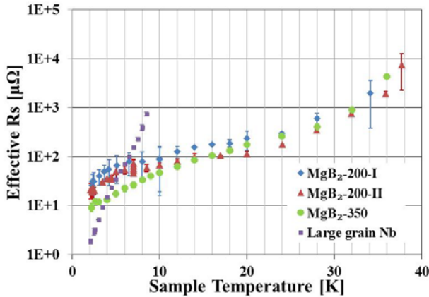
Figure 4: ◆ MgB 2 -200-I ▲ MgB 2 -200-II ● MgB 2 -350 Effective surface resistance of MgB 2 on sapphire substrate ■ Surface resistance of large grain Nb sample.
