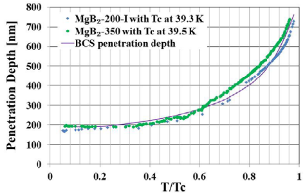
Figure 3: \blacklozenge MgB_2 -200-I with T_c 39.3 K \bullet MgB_2 -350 with T_c 39.5 K penetration depth versus sample temperature of MgB_2 on sapphire substrate – BCS penetration depth.
