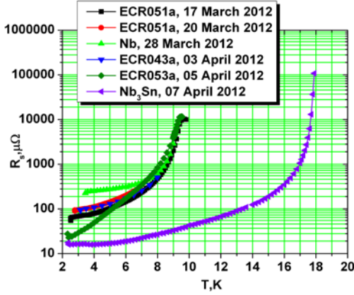
Figure 2: Measured surface resistance of several EC films, bulk Nb sample and Nb_3Sn sample.
