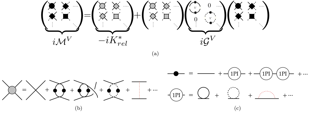
FIG. 1. a) Shown is the self consistent definition of \mathcal{M}^V , which is defined as the sum of all 2 \rightarrow 2 finite volume diagrams, Eq. 20. The solid lines denote two-particles in the “1” channel, dashed lines denote particle in the “2” channel. \mathcal{M}^V is written in terms of the c.m. kernel, K_{rel}^* , and the fully dressed single particle propagators. b) Shown is K_{rel}^* for the first channel, which is the sum of all two-particle irreducible s-channel diagrams. Explicitly shown are examples of diagrams that are included in the kernel: contact interactions, t- and u-channel diagrams and possible meson exchange diagrams, if allowed by the symmetries of the system of interest. If the two initial and final states of the kernel are baryons these exchange diagrams are presented, otherwise they are not allowed by G-parity. In general, all diagrams allowed by the underlying theory where the intermediate particles cannot all simultaneously go on-shell are absorbed into the kernel. As described in the text, in this study we are restricted to energies where only two-particle states are allowed to go on-shell. c) Shown is the definition of the fully dressed one particle propagator in terms of the one particle irreducible (1PI) diagrams.
