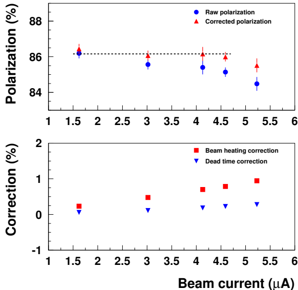
FIG. 3: Top: Electron beam polarization as determined by the Møller polarimeter as a function of current. The blue circle points are the raw measurements, while the red triangles include corrections for dead time and target heating effects. The dashed line is the best fit of the corrected data for all points at currents less than 5 \mu\text{A} . The average is 86.16 \pm 0.15\% (stat), with a \chi^2/\text{dof} of 0.5 (associated probability 0.69). Bottom: Size of correction vs. current, in percent. Red squares are the beam heating correction, while blue inverted triangles are the dead time correction.
