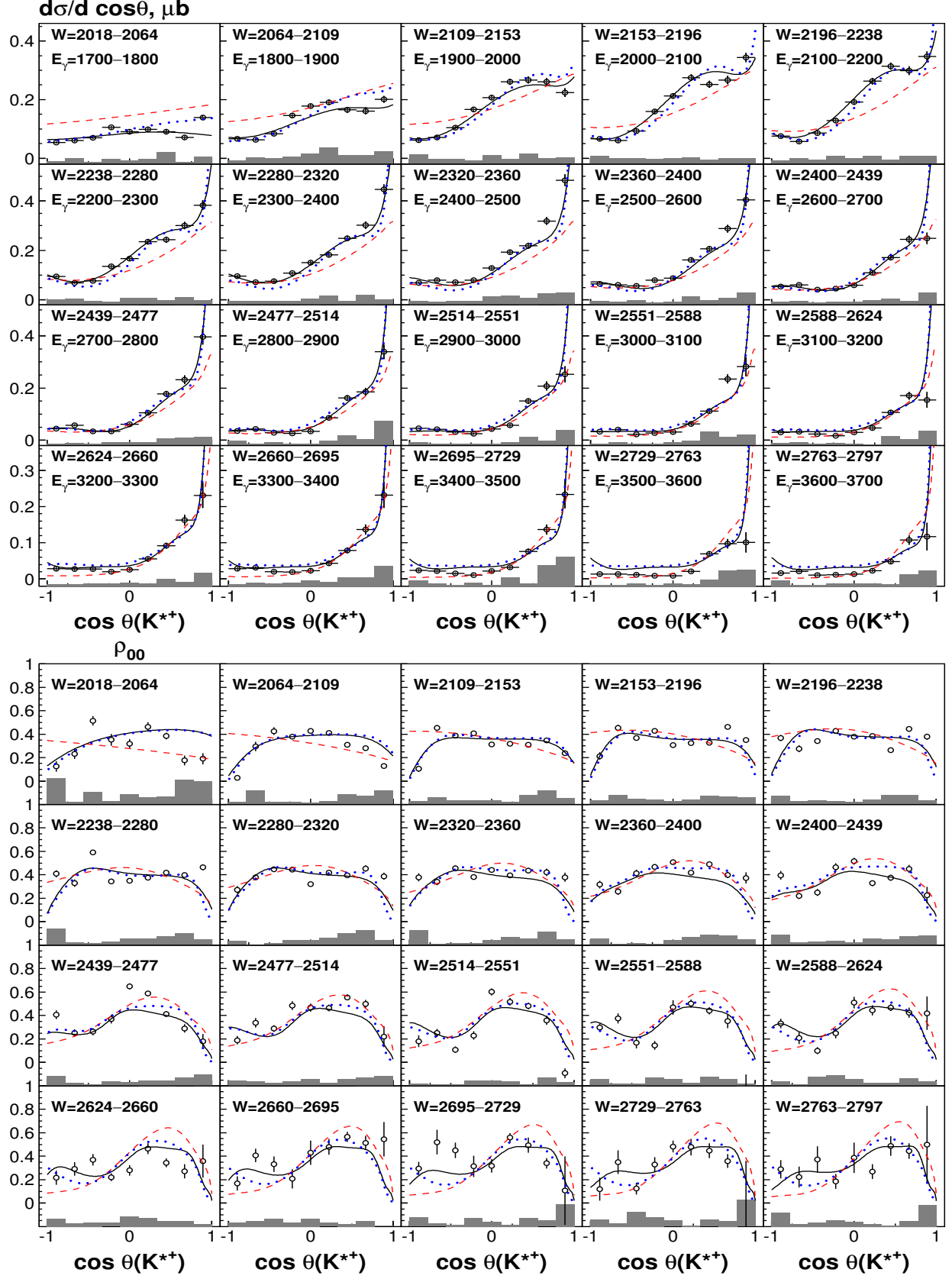
Figure 4: (Color online) Differential cross sections (top) and the \rho_{00} and density matrix elements (bottom) for the reaction \gamma p \rightarrow K^{*+}(892)\Lambda . The uncertainties contain statistical and systematic contributions. The solid curves represent the final BnGa fit, the dashed (red online) curves are fit with t-channel contributions only, the dotted (blue online) curves are fit with the new high-mass resonances omitted. The fits are restricted to invariant mass below 2.6 GeV, making curves at higher energies a prediction.
