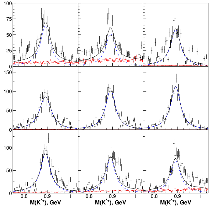
Figure 3: K_S^0 \pi^+ invariant mass distributions for 2200 < W < 2300 MeV and nine equidistant ranges in \cos\theta covering the full angular range, starting from backward angles in the top-left plot. The solid curve represents a fit with a Voigt function (dashed) plus background from a Monte Carlo simulation.
