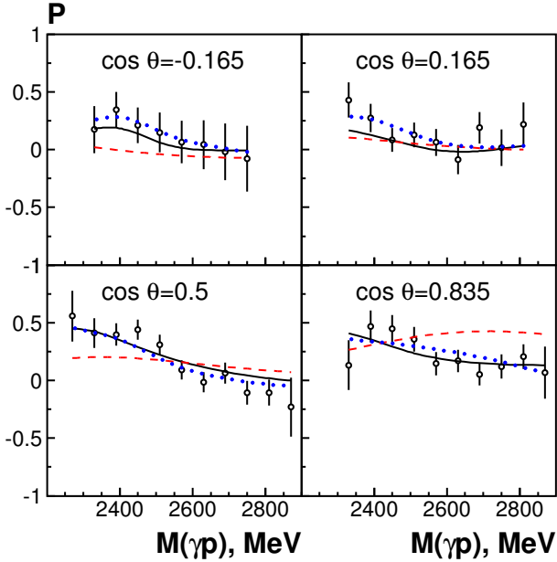
Figure 6: Recoil polarization of the \Lambda . The solid curves represent the final BnGa fit, the dashed (red online) curves a fit with t-channel contributions only, the dotted (blue online) curves a fit in which the new high-mass resonances are omitted. The fits are restricted to invariant mass below 2.6 GeV, making curves at higher energies a prediction.
