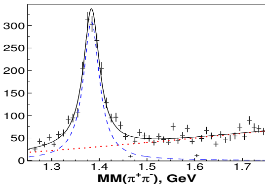
Figure 2: Example of a fit eliminating \Sigma(1385) .
