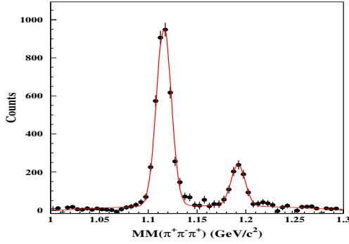
Figure 1: Example of two Gaussians plus a second order polynomial fit to the reconstructed \Lambda and \Sigma^0 missing mass peaks (adapted from Ref. [4]).
