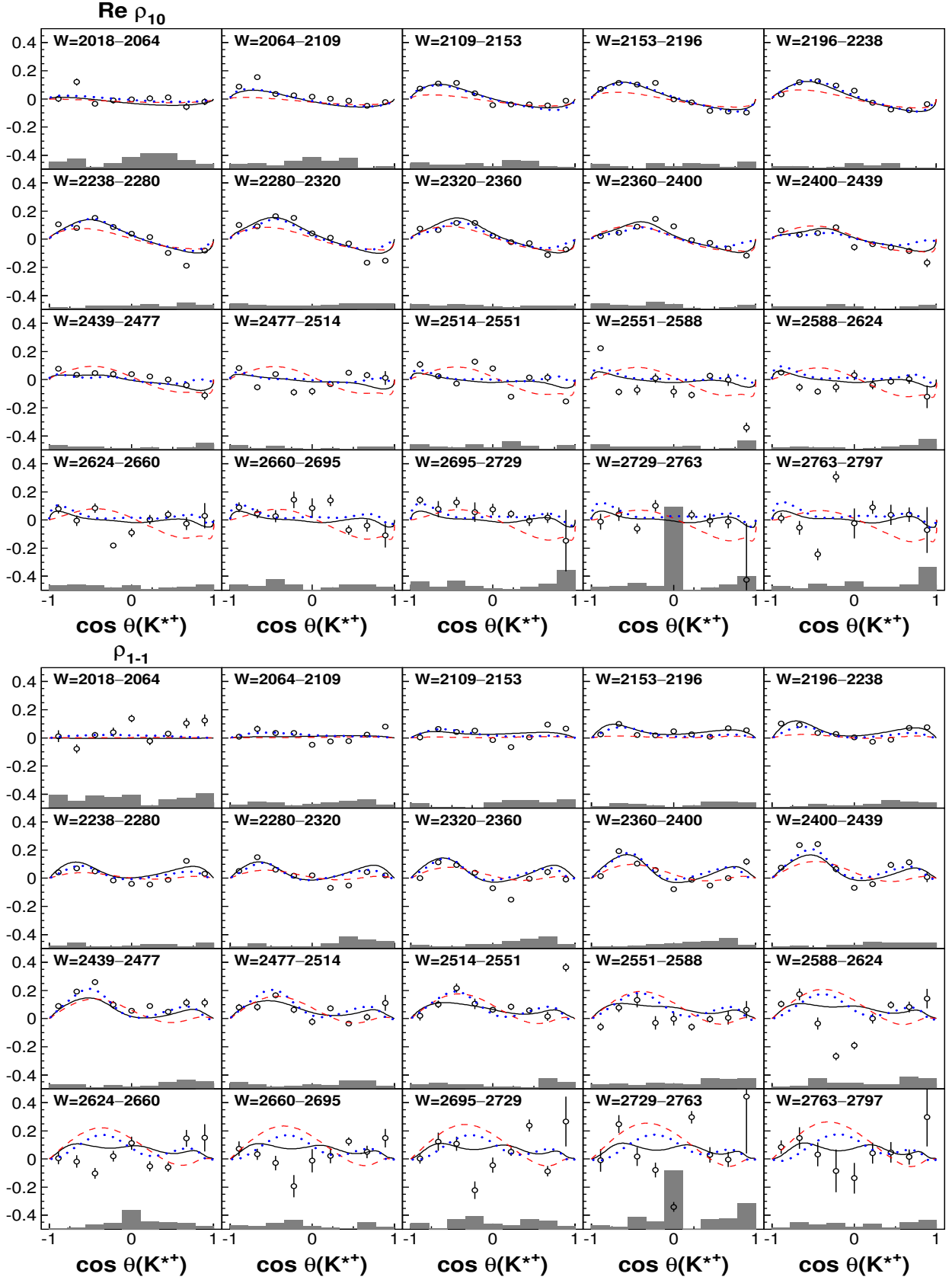
Figure 5: (Color online) The \rho_{10} (top) and \rho_{11} (bottom) density matrix elements for the reaction \gamma p \rightarrow K^{*+}(892)\Lambda . The uncertainties contain statistical and systematic contributions. The solid curves represent the final BnGa fit, the dashed (red online) curves a fit with t-channel contributions only, the dotted (blue online) curves a fit in which the new high-mass resonances are omitted. The fits are restricted to invariant mass below 2.6 GeV, making curves at higher energies a prediction.
