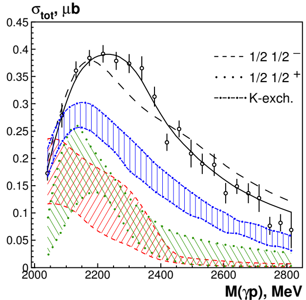
Figure 7: (Color online) The total cross section for the reaction \gamma p \rightarrow K^*\Lambda and the decomposition into its main components: the sum of t -channel exchanges, and the contributions from the I = 1/2 , J^P = 1/2^- and 1/2^+ partial waves. The hatched regions are labeled above, and the solid curve represents the final BnGa fit. The dashed line represents a fit which excludes the three high-mass resonances.
