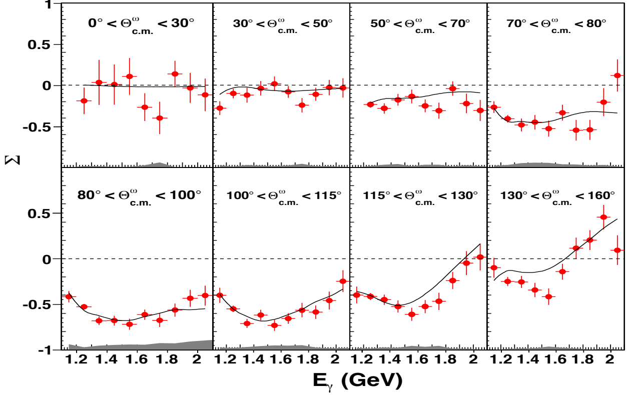
FIG. 9. Results for the beam asymmetry, \Sigma , using a linearly-polarized photon beam and an unpolarized target in the reaction \gamma p \rightarrow p\omega . The data are shown in bins of \Theta_{c.m.}^\omega versus incident-photon energy for the range of E_\gamma \in [1.1, 2.1] GeV. The gray band at the bottom of each panel represents the absolute systematic uncertainties of our results due to the background subtraction. The horizontal bars of the FROST data points indicate the angular range they cover. The black solid line denotes the BnGa-PWA solution [39].
