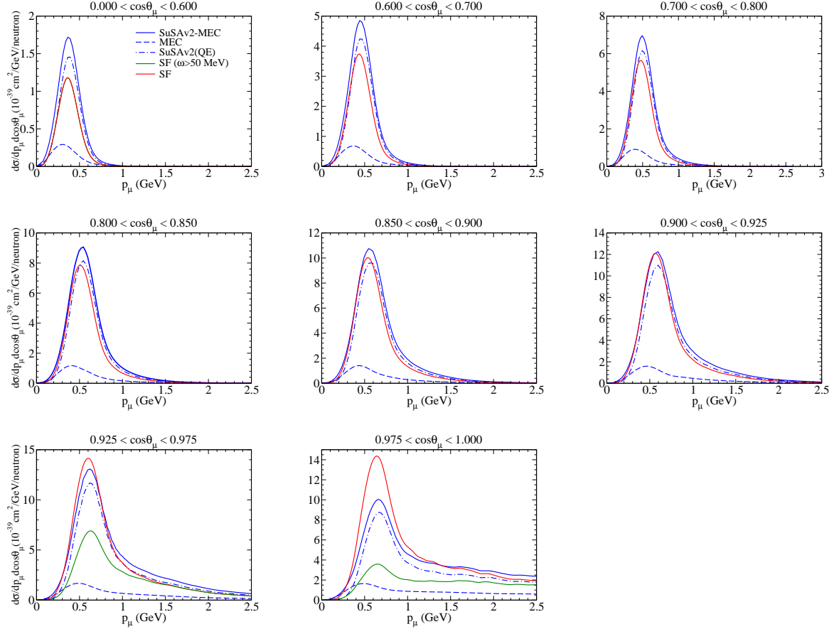
FIG. 9: (Color online) As for Fig. 3, but now for the \bar{\nu}_\mu CCQE process on oxygen. The SF results are also displayed. In the last two panels the SF result corresponding to \omega > 50 MeV is also shown (green curve).
