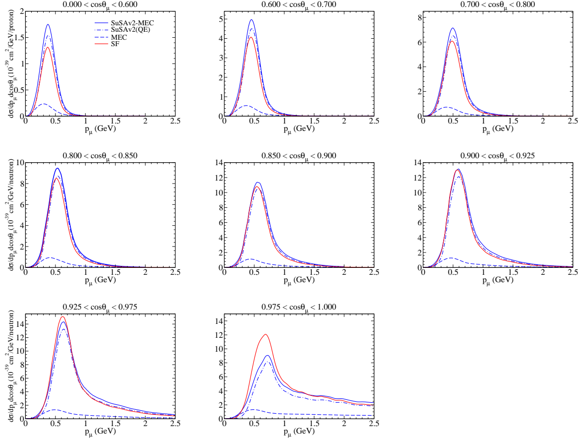
FIG. 10: (Color online) As for Fig. 3, but now for the \bar{\nu}_\mu CCQE process on water. The SF results are also displayed.
