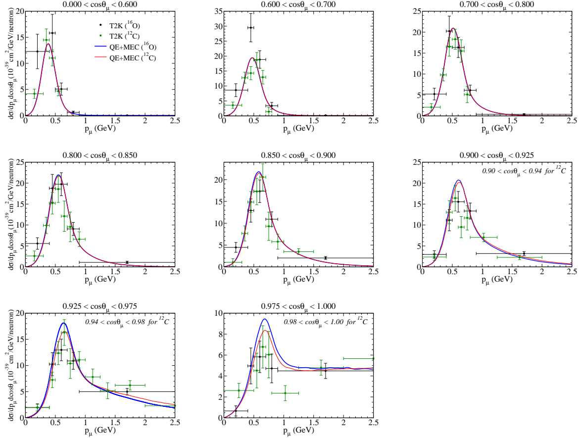
FIG. 5: (Color online) Similar to Fig. 3, but now including also the results corresponding to the T2K- \nu_\mu CCQE process on ^{12}\text{C} . The data are from [1, 41]
