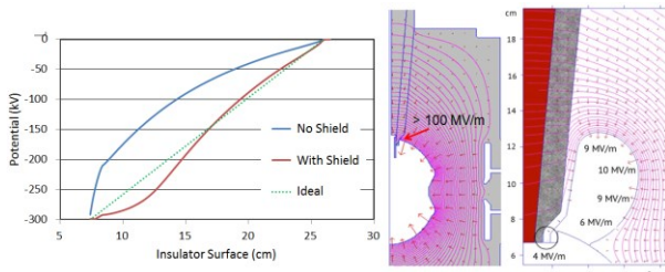
Figure 2: POISSON simulated electric field inside the photogun chamber with and without the shield electrode, and the potential along the length of the insulator surface.
