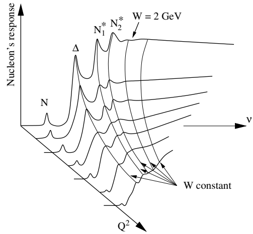
Figure 3: Response of the nucleon to the electromagnetic probe as a function of Q^2 and \nu . The \nu -positions of the peaks (N, \Delta(1232) 3/2^+, \dots ) change as Q^2 varies. (After [16].)
