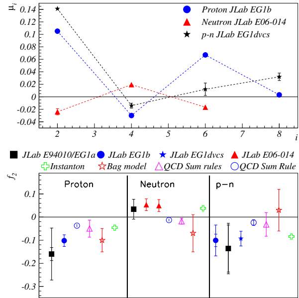
Figure 14: Top: coefficients \mu_i of the 1/Q^{2i-2} twist series vs i . The lines linking the points show the oscillatory behaviors. Bottom: twist-4 f_2 . Newer results (e.g. EG1dvcs) include the older data (e.g. EG1a).
