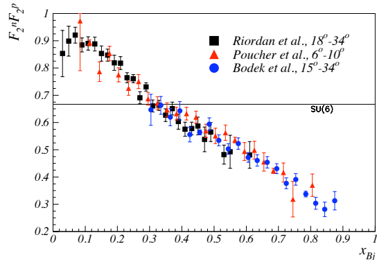
Figure 10: F_2^n/F_2^p SLAC data [317]. SU(6) predicts F_2^n/F_2^p = 2/3 .
