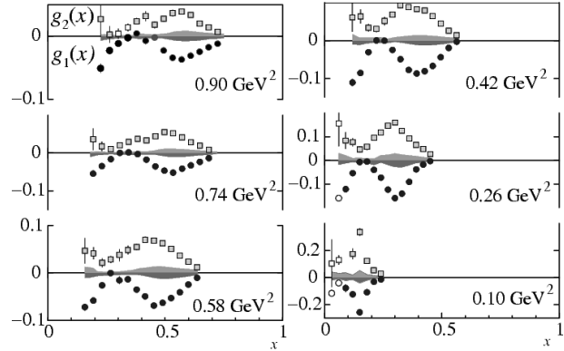
Figure 16: The symmetry between g_1 and g_2 . (JLab ^3\text{He} data from E94-010 [261].)
