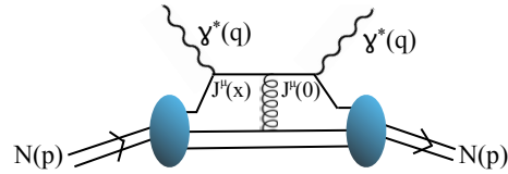
Figure 6: Forward virtual Compton amplitude with a Wilson line.
