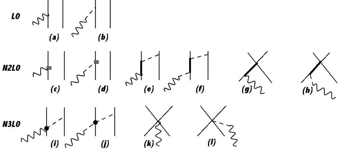
FIG. 1: Diagrams illustrating the contributions to the axial current up to N3LO ( Q^0 ). Nucleons, \Delta -isobars, pions, and external fields are denoted by solid, thick-solid, dashed, and wavy lines, respectively. The squares in panel (c) and (d) represent relativistic corrections, while the dots in panels (i) and (j) denote vertices implied by the \mathcal{L}_{\pi N}^{(2)} chiral Lagrangian. Only a single time ordering is shown. Note that the contact contributions in panels (g) and (h) vanish.
