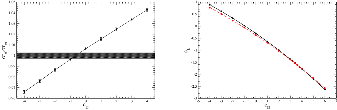
FIG. 2: Left panel: The calculated ratio GT_{th}/GT_{exp} as function of c_D (solid line; each point on this line reproduces the trinucleon binding energies). Right panel: The c_D - c_E trajectories obtained by fitting the experimental trinucleon binding energies (solid line) and nd doublet scattering length (dashed line) (the intercept of these two lines gives the c_D and c_E values that reproduce these two observables simultaneously). The NV2+3-Ia chiral interactions are used here for illustration. The values of 8.475 MeV and 7.725 MeV, and 0.645 \pm 0.010 fm [42] are used for the {}^3\text{H} and {}^3\text{He} binding energies, and nd scattering length, respectively. Note that these energies have been corrected for the small contributions (+7 keV in {}^3\text{H} and -7 keV in {}^3\text{He} ) due to the n - p mass difference [43]. The band (left panel) results from experimental uncertainty GT_{exp} , which has conservatively been doubled.
