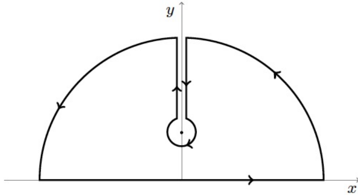
FIG. 3: Integration contour.
