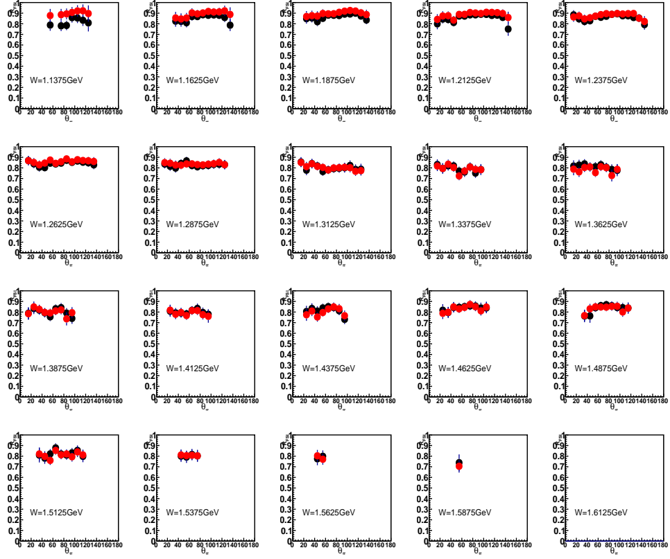
Figure 6.11: R_{FSI} versus \theta_{\pi^-}^* distributions example for individual W bins, which are increasing by 0.025 GeV in the range of 1.125 \text{ GeV} < W < 1.6 \text{ GeV} for 0.8 \text{ GeV}^2 < Q^2 < 1.0 \text{ GeV}^2 . The red and black points correspond to R_{FSI} binned in W_i and W_f , respectively.
