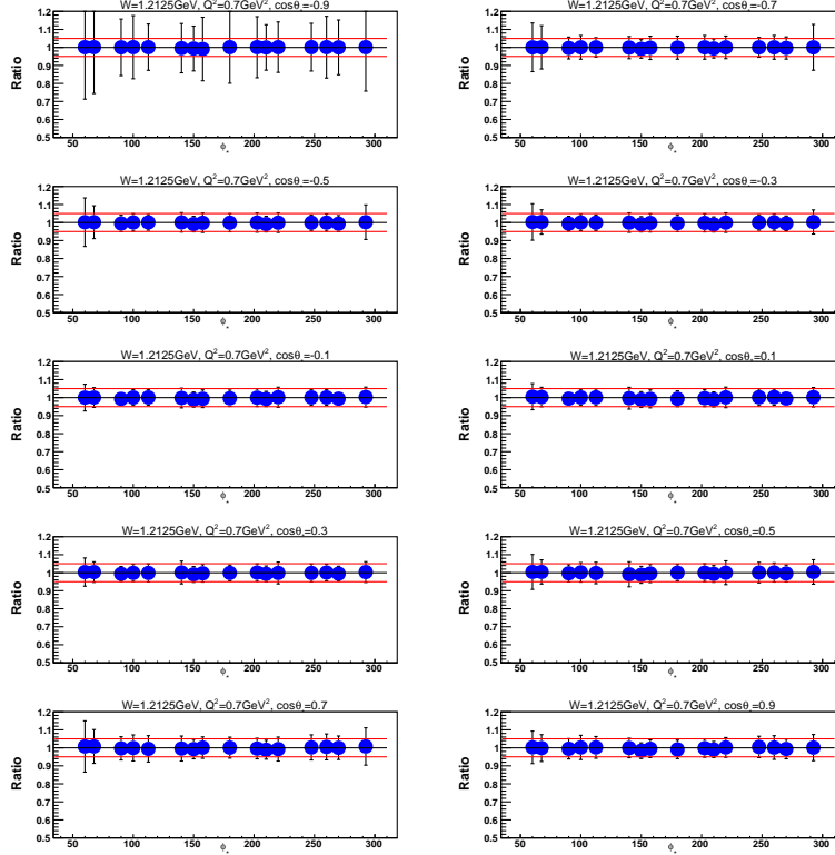
Figure 6.7: The ratios of R_{FSI}(W_i, Q^2, \cos \theta_{\pi^-}^*, \phi_{\pi^-}^*) over R_{FSI}(W_i, Q^2, \cos \theta_{\pi^-}^*) are represented by Blue points for different \phi_{\pi^-}^* at 1.2 \text{ GeV} < W_i < 1.225 \text{ GeV} and 0.6 \text{ GeV}^2 < Q^2 < 0.8 \text{ GeV}^2 . The individual plot shows the ratios for different \cos \theta_{\pi^-}^* bins. The three lines from bottom to top correspond to 0.95, 1, and 1.05, respectively.
