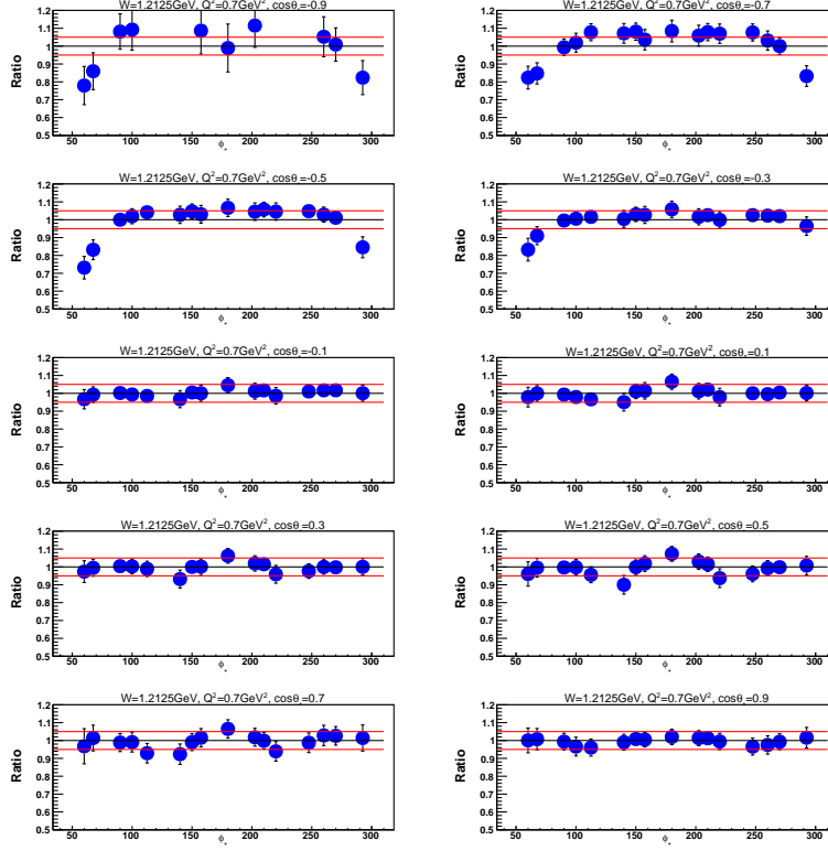
Figure 6.8: The ratios of R_{FSI}(W_i, Q^2, \cos \theta_{\pi-}^*, \phi_{\pi-}^*) over R_{FSI}(W_i, Q^2, \cos \theta_{\pi-}^*) are represented by Blue points for different \phi_{\pi-}^* at 1.2 \text{ GeV} < W < 1.225 \text{ GeV} and 0.6 \text{ GeV}^2 < Q^2 < 0.8 \text{ GeV}^2 . The individual plot shows the ratios for different \cos \theta_{\pi-}^* bins. The three lines from bottom to top correspond to 0.95, 1, and 1.05, respectively.
