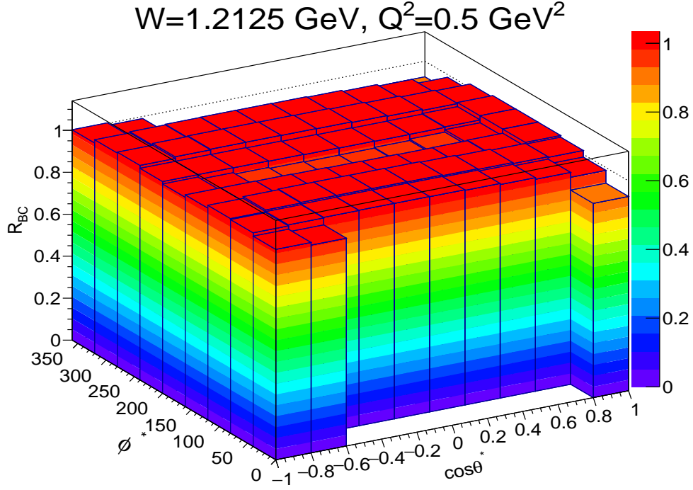
Figure 5.3: Bin centering corrections R_{BC} as a function of \cos\theta^* and \phi^* in the W = 1.2125 GeV and Q^2 = 0.5 GeV 2 bin.
