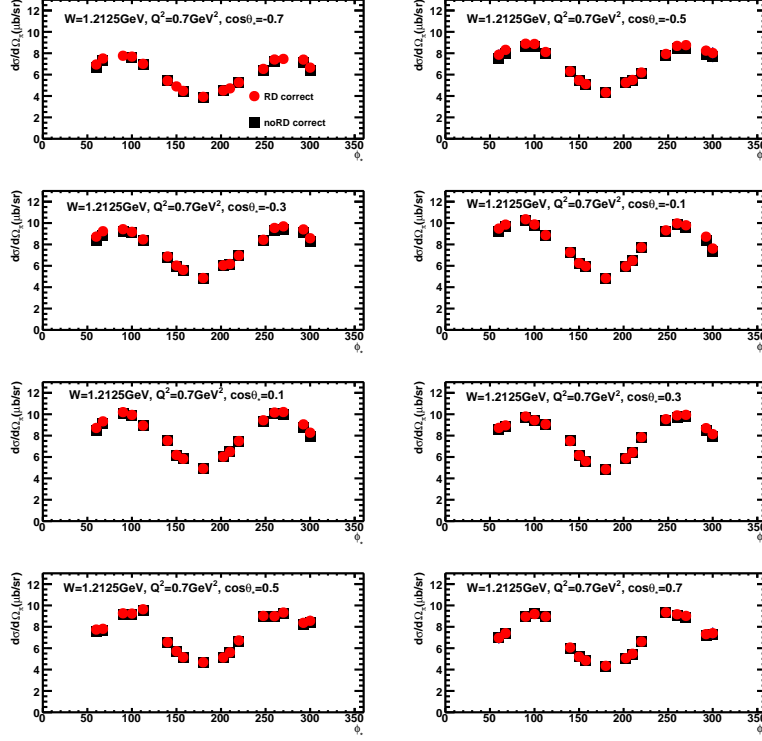
Figure 6.19: The \phi_{\pi^*}^* – dependence of the exclusive cross sections with and without radiative correction are marked as red points and black squares, respectively for an example at W = 1.2125 GeV and Q^2 = 0.7 GeV 2 . The individual plots correspond to different \cos \theta_{\pi^*}^* – bins.
