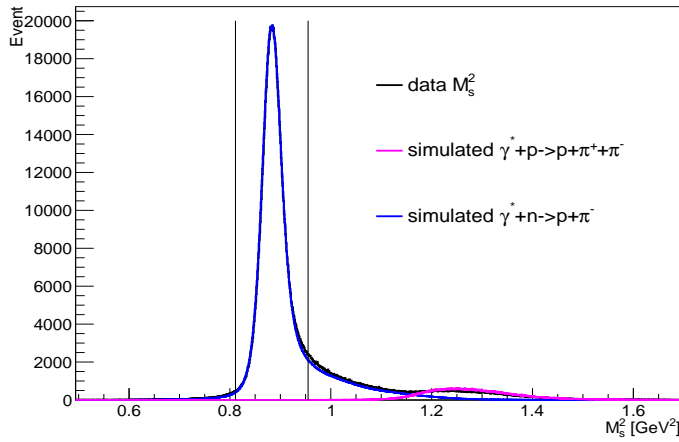
Figure 5.7: M_s^2 distributions for measured (black) and simulated \gamma^* n(p) \rightarrow p\pi^-(p) (blue), as well as simulated \gamma^* p \rightarrow p\pi^-\pi^+ events are plotted with the M_s^2 cut limits.
