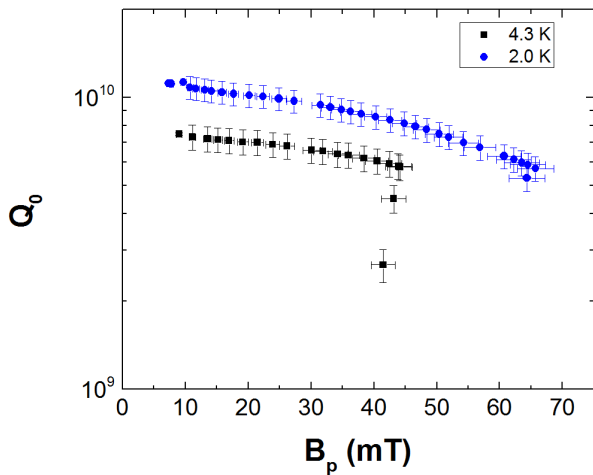
Figure 2: Q_0(B_p) measured at 4.3 K and 2.0 K after the first \text{Nb}_3\text{Sn} coating 1 . The cavity was limited by anomalous heating at 4.3 K and by quench at 2.0 K.
