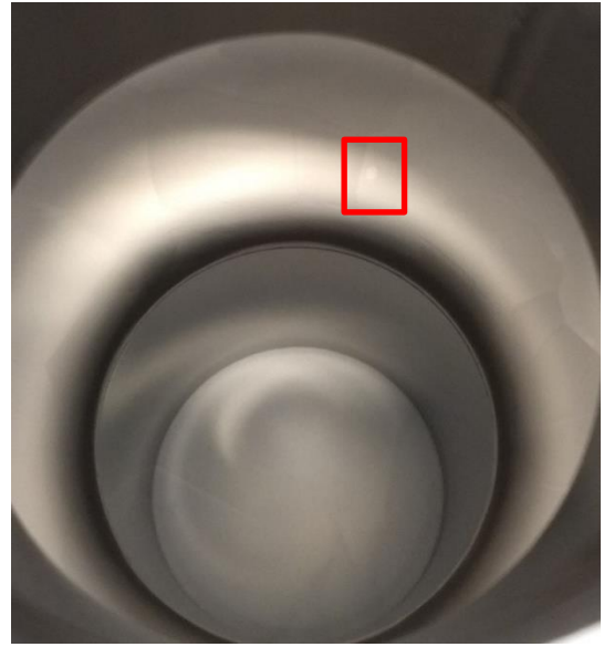
Figure 3: A picture of SC-IB interior after second \text{Nb}_3\text{Sn} coating. Note the shiny spot marked by red rectangle.
