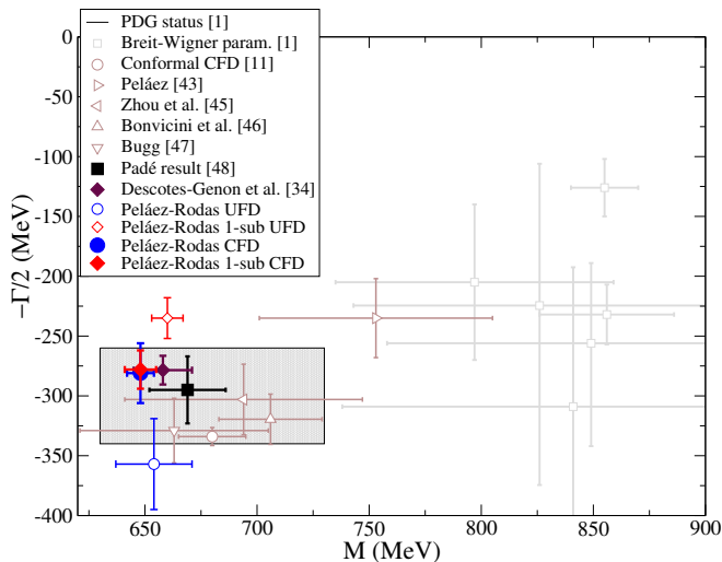
FIG. 1. K_0^*(700) pole positions. We also show the results using Roy-Steiner equations, using as input our UFD or CFD parameterizations. Red and blue points use for F^- a once-subtracted or an unsubtracted dispersion relation, respectively. This illustrates how unstable pole determinations are when using simple fits to data. Only once Roy-Steiner Eqs. are imposed as a constraint, both pole determinations fall on top of each other. This final pole position is the main result of this work.
