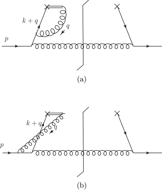
FIG. 3: Graphs (a) and (b), along with their Hermitian conjugates, are needed in general for gauge invariance. Analogous graphs are also needed for the collinear QS function.
