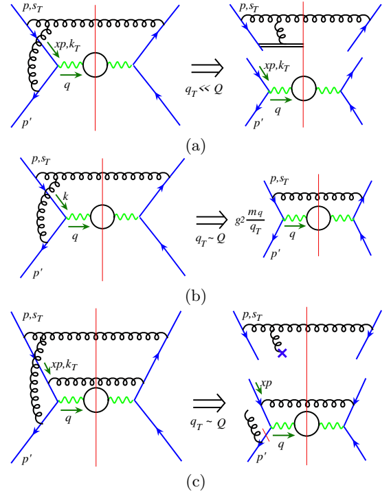
FIG. 1: Low order diagrams for A_N of Drell-Yan lepton pair production by hard quark-antiquark annihilation: (a) TMD factorization when k_T \sim Q_T \ll Q = \sqrt{q^2} . (b) fixed-order pQCD calculation when Q_T \sim Q . (c) Twist-3 collinear factorization when k_T \ll Q_T \sim Q .
