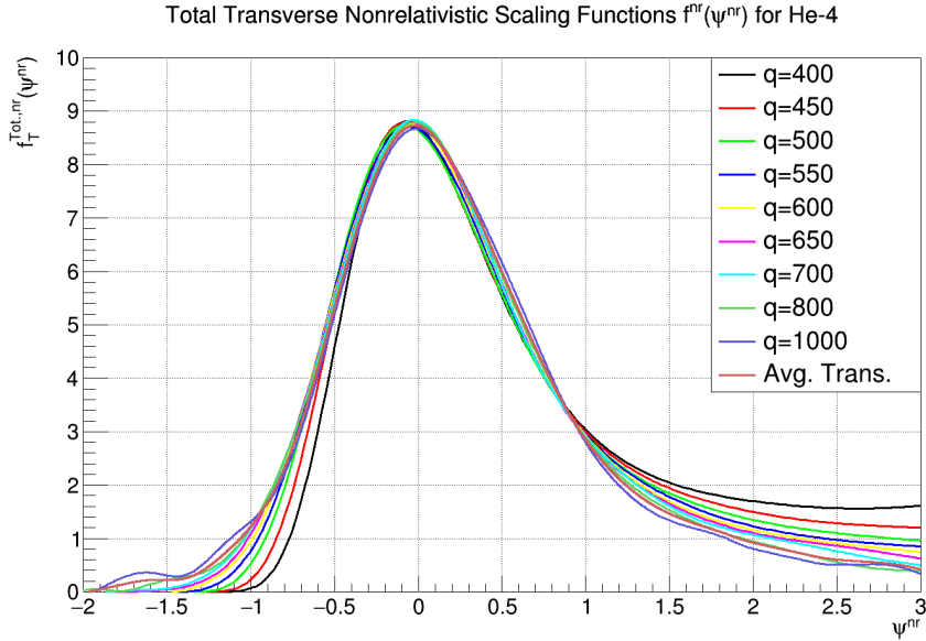
FIG. 2. Transverse scaling functions for {}^4\text{He} with one- and two-nucleon currents. Figure from Barrow et al. [18].
