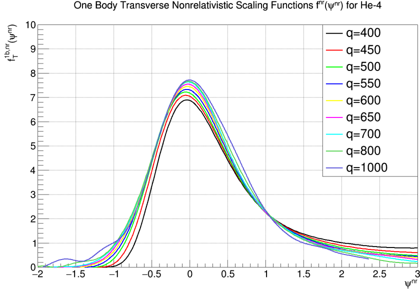
FIG. 1. Transverse scaling functions for {}^4\text{He} with single-nucleon currents only. Figure from Barrow et al. [18].
