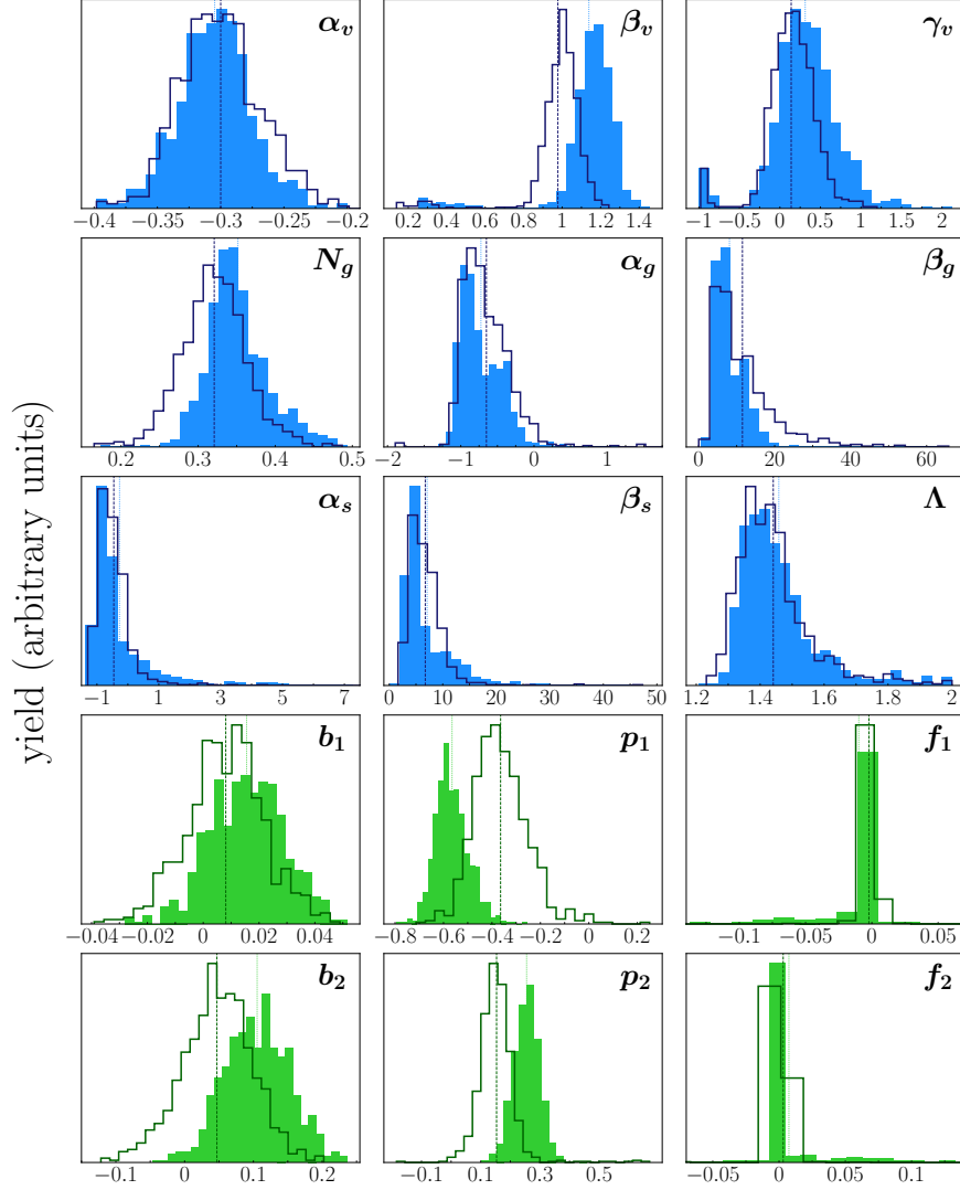
FIG. 2. Distributions of the free parameters describing PDF shapes \{\alpha_v, \beta_v, \gamma_v; N_g, \alpha_g, \beta_g; \alpha_s, \beta_s\} and the ultraviolet cutoff mass \Lambda in the N \rightarrow \pi N splitting function (blue histograms), and the intrinsic lattice systematic parameters \{b_1, p_1, f_1; b_2, p_2, f_2\} (green histograms) from the Monte Carlo fits, in arbitrary units. Both the NLO (outlined histograms) and NLO+NLL DY (filled histograms) analyses are shown, with the vertical dotted lines giving the mean values of the parameters.
