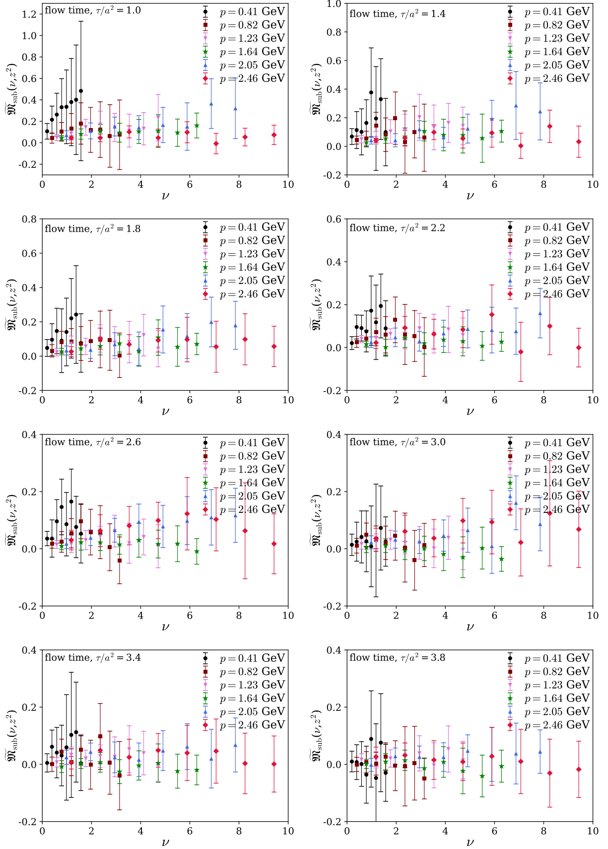
FIG. 8. The reduced matrix elements, \widetilde{\mathcal{M}}_{\text{sub}}(\nu, z^2) with respect to the Ioffe-time for different flow times. Starting from the top-left to bottom-right panels, the reduced matrix elements are shown for \tau/a^2 = 1.0 to 3.8.
