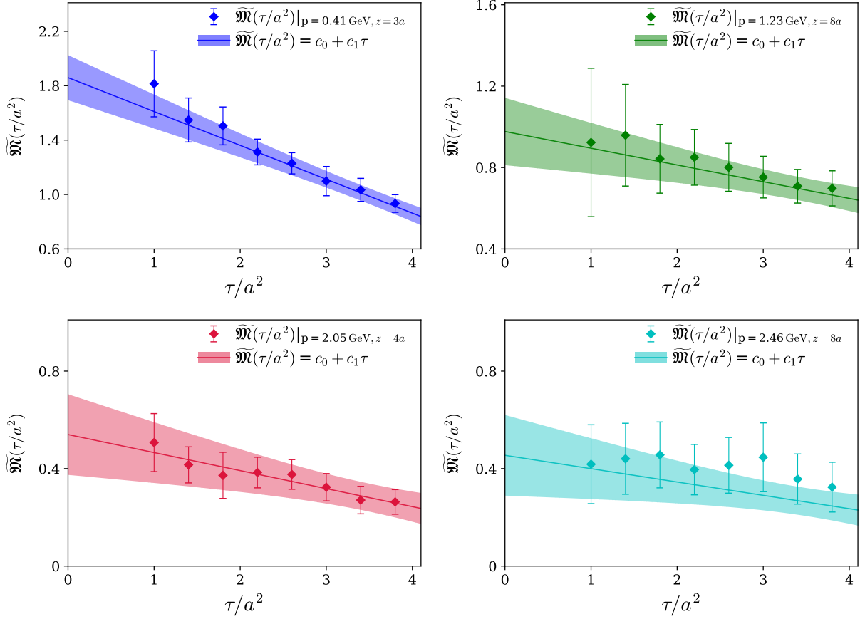
FIG. 5. Arbitrary examples of reduced matrix elements \widetilde{\mathfrak{M}}(\tau/a^2) extrapolated to the \tau \rightarrow 0 limit for different nucleon momenta and field separations. The functional form used to fit the reduced matrix elements is: \widetilde{\mathfrak{M}}(\tau/a^2) = c_0 + c_1\tau . The top-left panel shows the fit for p = 1 \times \frac{2\pi}{aL} = 0.41 GeV and z = 3a . The top-right panel shows the fit for p = 3 \times \frac{2\pi}{aL} = 1.23 GeV and z = 8a . The bottom-left panel shows the fit for p = 5 \times \frac{2\pi}{aL} = 2.05 GeV and z = 4a . The bottom-right panel shows the fit for p = 6 \times \frac{2\pi}{aL} = 2.46 GeV and z = 8a .
