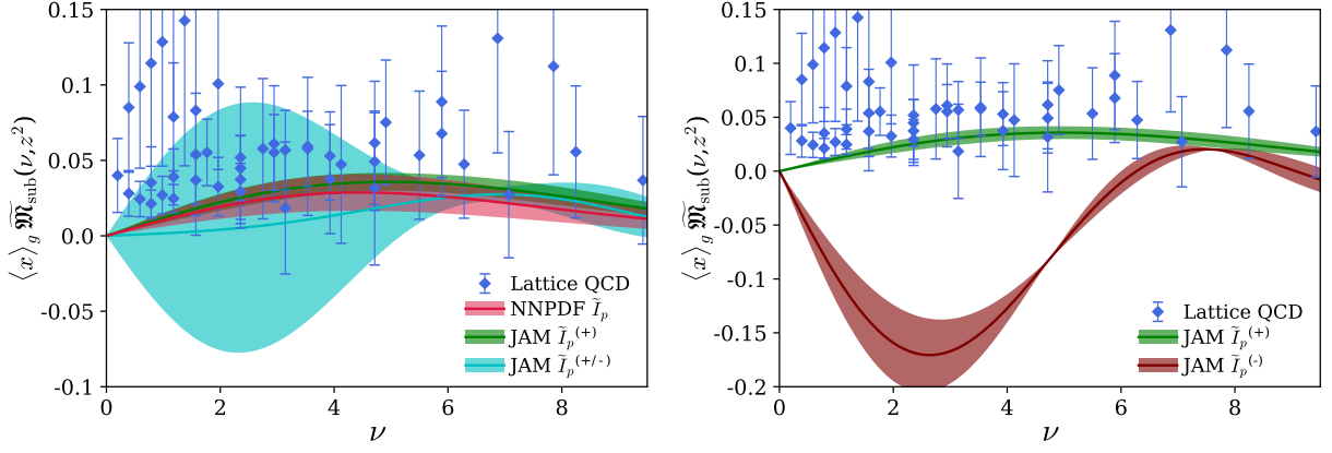
FIG. 10. A comparison between the lattice reduced Ioffe-time pseudo-distribution \widetilde{\mathcal{M}}(\nu, z^2) in the zero flow-time limit obtained through the subtraction method using the p = 0 matrix elements, and gluon helicity ITD constructed from global fits of PDFs. The lattice data points are the same as in Fig. 9, plotted on a smaller vertical scale for better comparison with the phenomenological ITD bands. In the left plot, the red band denotes the ITD constructed from the gluon helicity distribution by the NNPfD collaboration. The green band labeled by \tilde{\mathcal{I}}_p^{(+)} and the cyan band labeled by \tilde{\mathcal{I}}_p^{(+/-)} represent the gluon helicity ITD determined by the JAM collaboration with and without the positivity constraint on the gluon helicity PDF, respectively. On the right plot, the gluon helicity ITDs for positive and negative helicity PDFs are compared with the lattice data. The green band labeled by \tilde{\mathcal{I}}_p^{(+)} and the maroon band labeled by \tilde{\mathcal{I}}_p^{(-)} represent the gluon helicity ITD determined by the JAM collaboration associated with the positive and negative gluon helicity PDF solutions, respectively.
