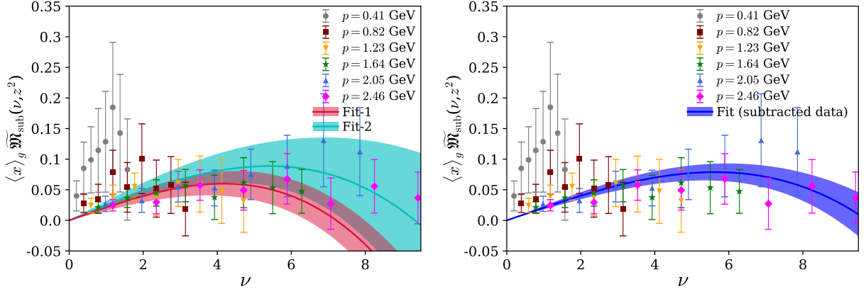
FIG. 9. The lattice data points represent the reduced Ioffe-time pseudo-distribution, \widetilde{\mathcal{M}}(\nu, z^2) in the zero flow-time limit obtained through the subtraction method using p = 0 matrix elements. The lattice data points and the fit bands are normalized using the gluon momentum fraction, \langle x \rangle_g from [17]. (Left panel) The red and cyan bands represent the target mass corrected reduced Ioffe-time pseudo-distribution using the fit of moments in Sec. IV A. (Right panel) The blue band is a fit to the subtracted pseudo-ITD using the functional form in Eq. (20) with a_0, a_1, b_1 as fit parameters and b_0 = 0 fixed by construction.
