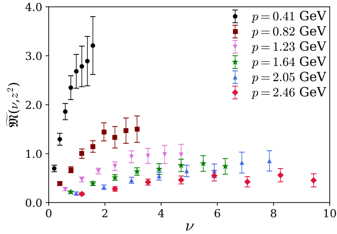
FIG. 6. The reduced Ioffe-time pseudo-distribution \widetilde{\mathfrak{M}}(\nu, z^2) in the zero flow-time limit.
