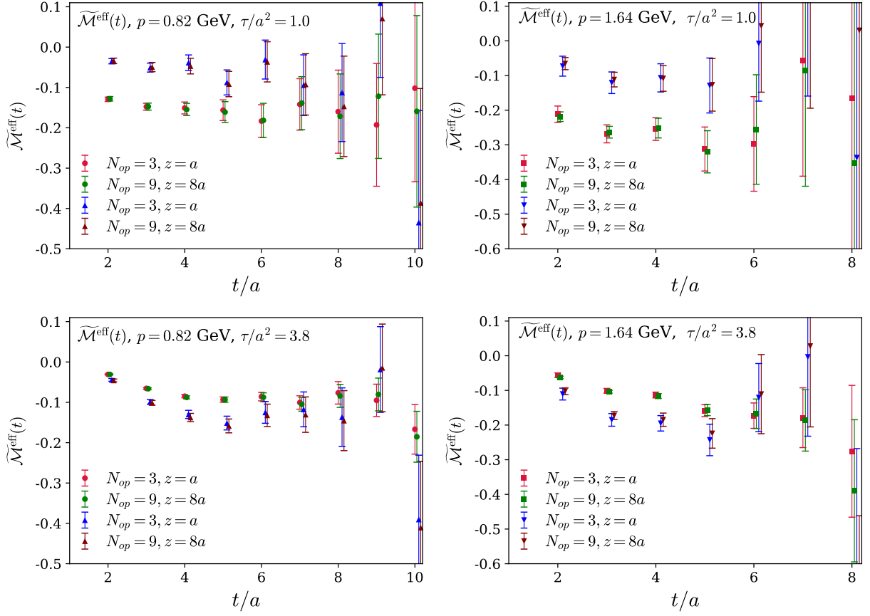
FIG. 11. Comparison plots of a few polarized gluon matrix elements \widetilde{M}^{\text{eff}}(t) between 3 and 9 different number of interpolators as illustrated in Table II. The smaller basis of interpolators is used in this work based on the observation that the smaller basis of interpolators reproduces the matrix elements constructed with the larger basis of interpolators through the sGEVP analysis.
