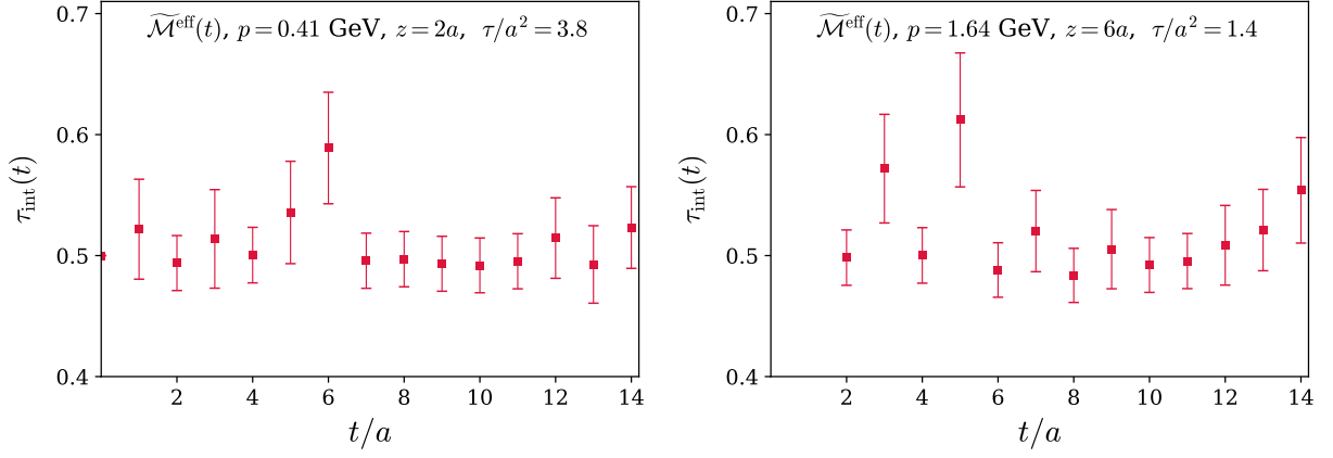
FIG. 12. The integrated autocorrelation time of the gluonic bare effective matrix elements. The left panel has \tau_{\text{int}} for the nucleon momentum, p = \frac{2\pi}{aL} = 0.41 \text{ GeV} , the field separation, z = 2a = 0.188 \text{ fm} , at the flow time, \tau/a^2 = 3.8 , plotted with respect to the source-sink separation of the nucleonic two-point correlators and the right panel has \tau_{\text{int}} for the nucleon momentum, p = 4 \times \frac{2\pi}{aL} = 1.64 \text{ GeV} , the field separation, z = 6a = 0.564 \text{ fm} , at the flow time, \tau/a^2 = 1.4 .
