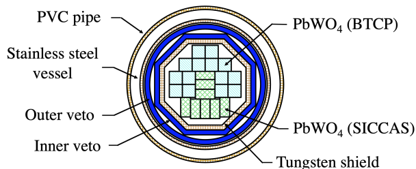
FIG. 2. Sketch of the “BDX-MINI” detector. The detector is located inside a well, illustrated in Fig.1, whose wall is shown as the outer PVC cylinder in this sketch. The detector package fits inside the stainless steel vessel.
