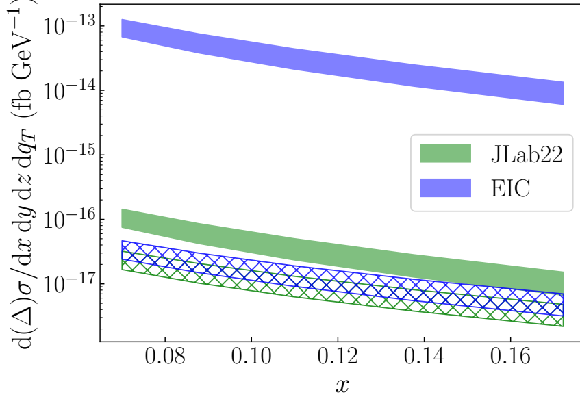
FIG. 7. Unpolarized (solid bands) and polarized (hatched bands) differential cross sections calculated for semi-inclusive \pi^+ production at the (x, Q^2, z, q_T) kinematics displayed in Fig. 5 for JLab with a 22 GeV beam energy (green bands) and EIC center of mass energy \sqrt{s} = 140 GeV (blue bands).
